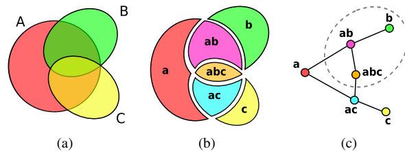
Figure 2: From the Euler diagram to the intersection graph. (a) the original diagram. (b) individuation of the diagram zones. (c) the resulting intersection graph. The dashed line is not part of the graph, but shows how to reverse the procedure. For drawing the boundary of the class B we need to enclose the nodes b, ab, abc and intersect the edges (a, ab), (ac, abc) .
