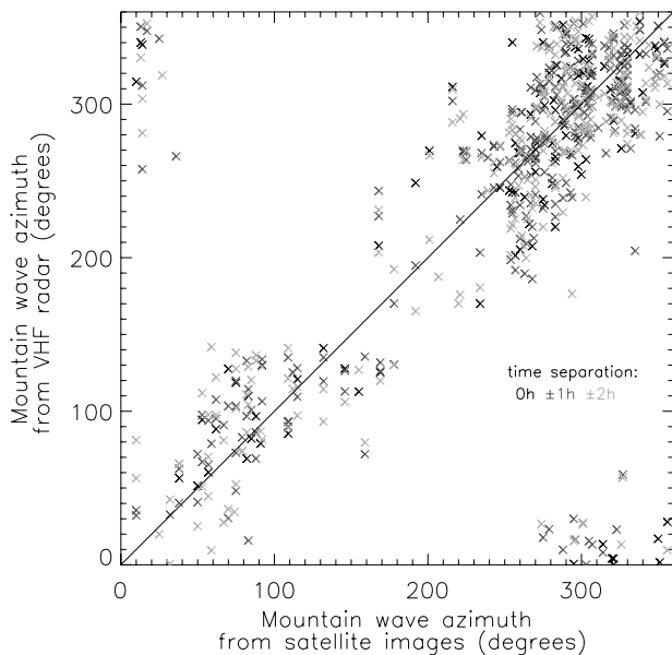
Fig. 12. Mountain-wave azimuths from VHF radar and satellite images, 1996–2006. Wave azimuth from satellite is perpendicular to cloud lines, pointing upwind. Time separation between radar and satellite data is 0, 1 or 2 h. The diagonal line is for equal radar and satellite azimuths.
