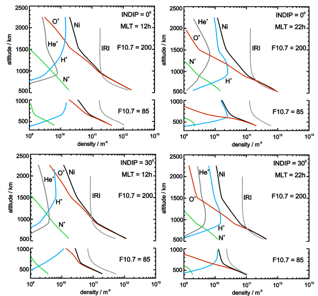
Fig. 8. Equinoxial daytime and nighttime vertical profiles of absolute densities for the four main ions as derived from the proposed N_e model and from the relative ion composition TTS model. The total ion density N_i following from our model and the IRI (Bilitza, 1990) values are shown.
