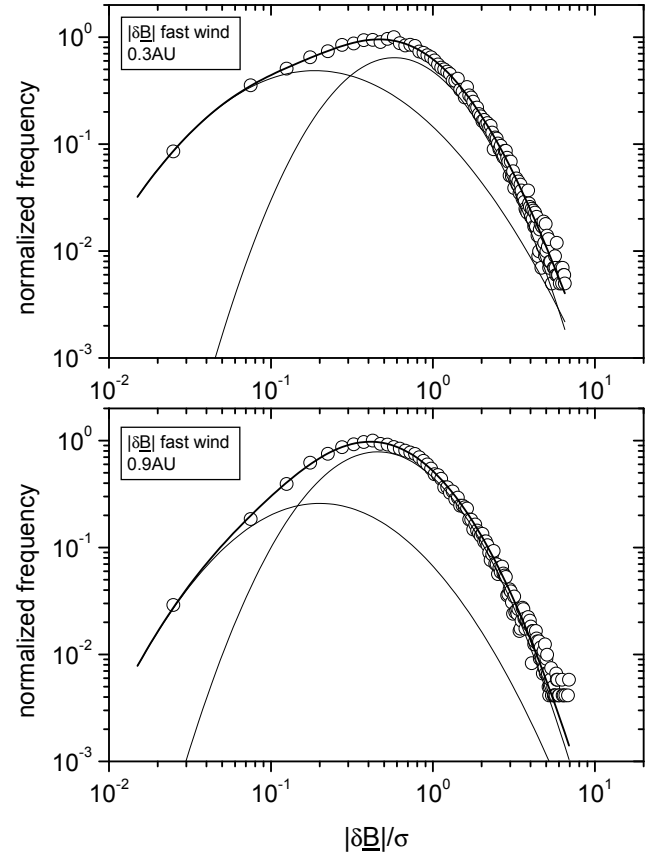
Fig. 8. PDFs of vector displacements |\delta \underline{B}| normalized to \sigma at 0.3 and 0.9 AU, for a fast wind, are shown in the top and bottom panels, respectively. The two thin solid curves refer to as many lognormals contributing to form the thick solid curve which best fit the distribution. Parameters relative to the fit are reported in Table 2.
