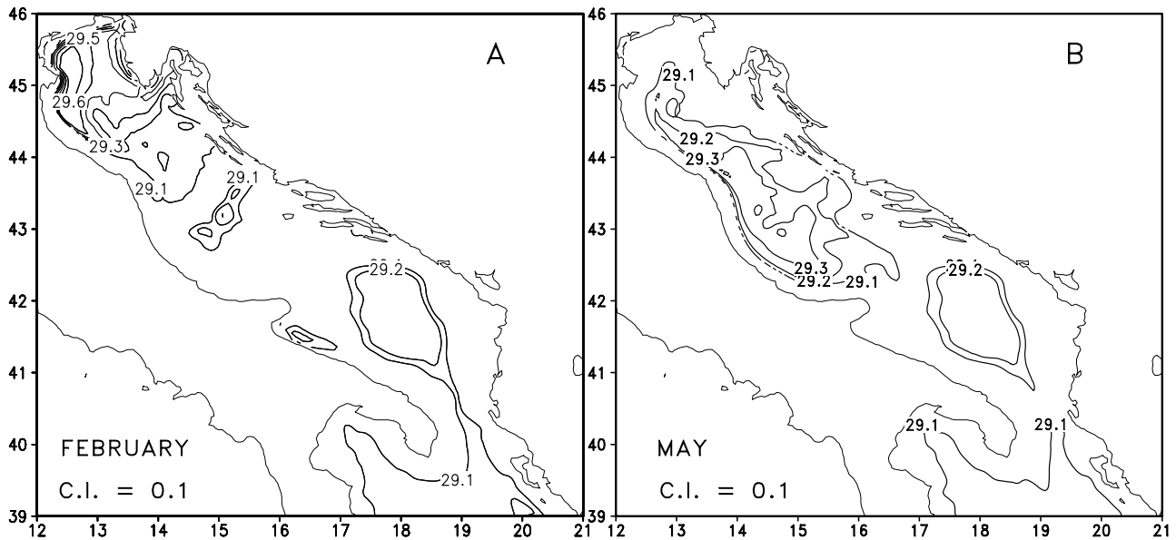
Fig. 11. Adriatic Intermediate Model (AIM). Bottom \sigma_\theta distribution. (A): February, (B): May. Contour interval is 0.1 \text{ kg/m}^3 . For clarity, \sigma_\theta values lower than 29.1 \text{ kg/m}^3 have been masked out.
