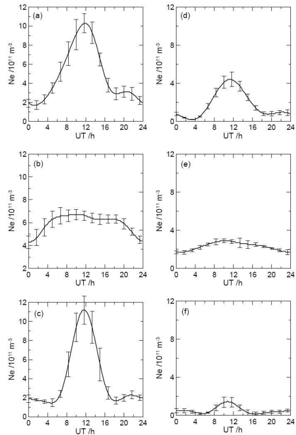
Fig. 4. Diurnal variation of mean N_e at 290 km around solar maximum (a, b and c) and at 230 km around solar minimum (d, e and f). (top panel: equinox; middle panel: summer; bottom panel: winter) (units: 10^{11} \text{ m}^{-3} ).
