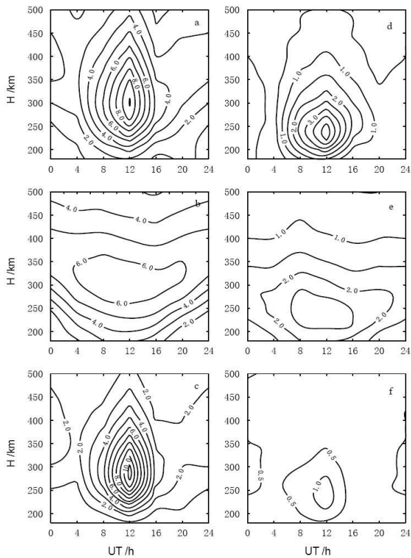
Fig. 3. 2-D distributions of mean N_e versus UT and height H around solar maximum (a, b and c) and solar minimum (d, e and f). (top panel: equinox; middle panel: summer; bottom panel: winter) (units: 10^{11} \text{ m}^{-3} ).
