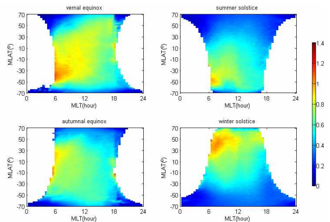
Fig. 4. Distribution of the columnar [O/N2] centered at equinox and solstice during the year 2003.
