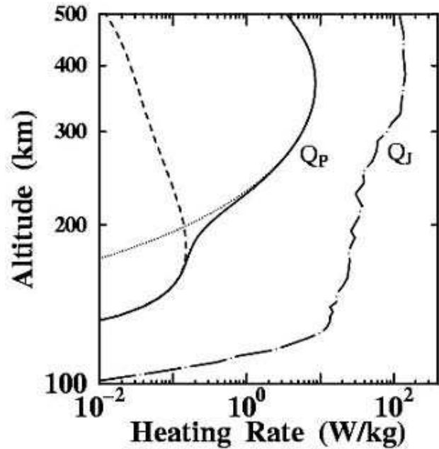
Fig. 9. The calculated heating rates (W/kg) due to precipitating electrons (dotted line), protons (dashed line), both particles (solid line labeled Q_P ), and \sigma_p E^2 / \rho at 09:10 UT derived from the ESR observations (dashed-dotted line labeled Q_J ).
