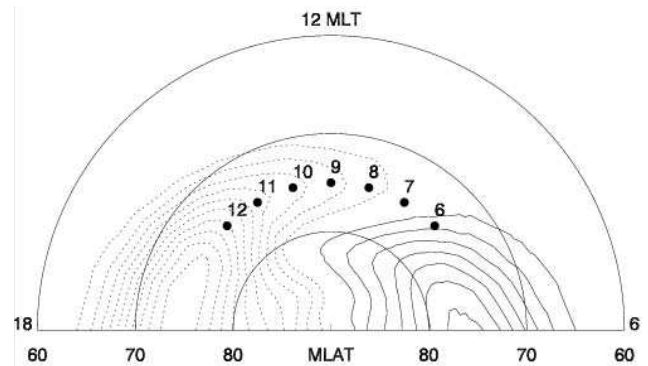
Fig. 3. High latitude electric potential calculated by using the Heppner-Maynard electric convection field model in the condition that IMF B_y and B_z are negative. The locations of the ESR site during 06:00–12:00 UT are marked by circle dots with numbers indicating the universal time.
