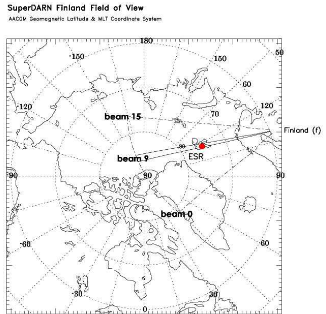
Fig. 2. Location of the ESR site at Longyearbyen (circle dot) and the field of view of the CUTLASS Finland radar in the geomagnetic latitude and MLT coordinate system. The field of view of the CUTLASS Finland radar consists of 16 beams (Beam 0–15), with Beam 9 over the ESR site.
