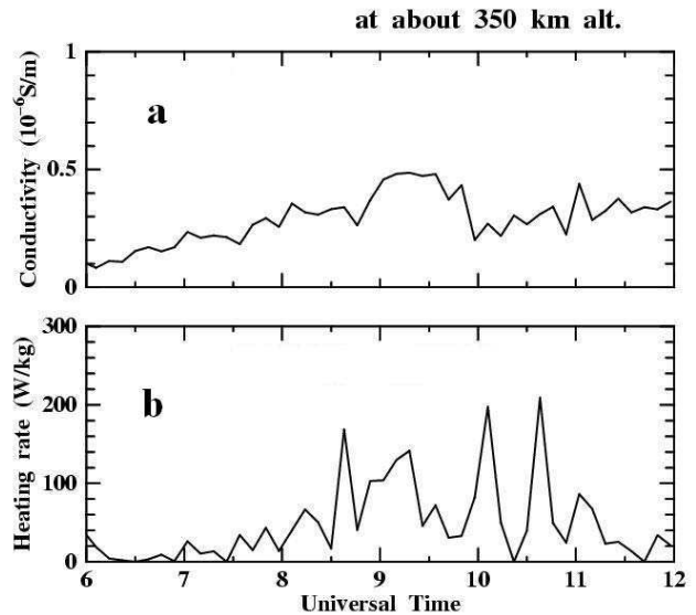
Fig. 7. (a) The Pedersen conductivity, \sigma_p and (b) passive energy deposition rate, \sigma_p E^2/\rho , at about 350 km altitude obtained from the ESR observations during 06:00–12:00 UT. These are the same as those shown in Fig. 6 except for line plots at a specific height.
