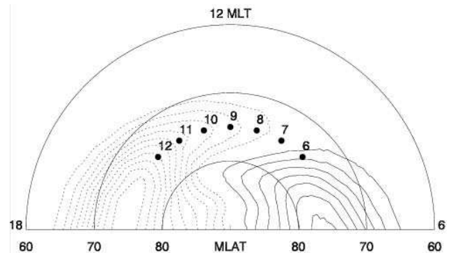
Fig. 3. High latitude electric potential calculated by using the Heppner-Maynard electric convection field model in the condition that IMF B_y and B_z are negative. The locations of the ESR site during 06:00–12:00 UT are marked by circle dots with numbers indicating the universal time.
