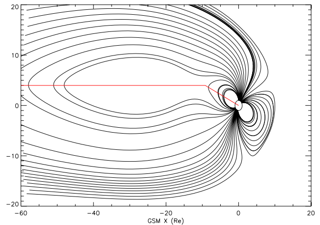
Fig. 2. A noon-midnight cut through the magnetosphere around the June solstice. The black lines show the field topology derived from the Tsyganenko 2005 model. The red line shows how the neutral sheet location can be represented by a simple hinge model. One segment lies in the geodipole equatorial plane while the other lies parallel to the ecliptic; the two are linked by a hinge at geocentric distance of 10 R_E .
