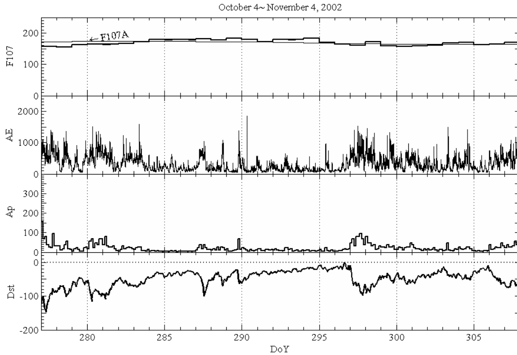
Fig. 1. The solar geophysical conditions during the long-duration Millstone Hill ISR experiment from 4 October and 4 November 2002.
