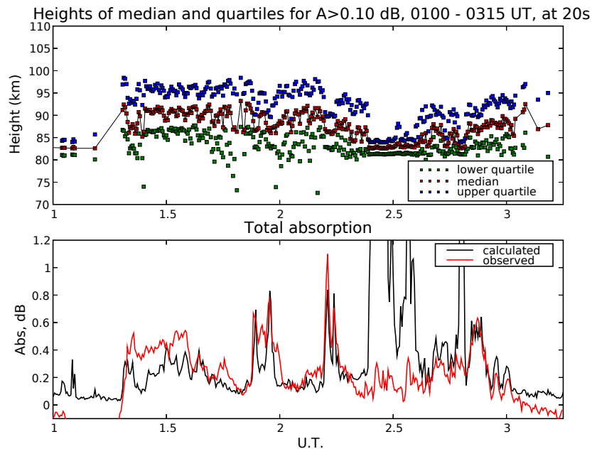
Fig. 10. The absorption layer for 01:00–03:15 UT (01.00–03.25 UT) on 2 July. The upper panel shows the calculated median and quartiles, and the lower one compares the calculated 38.2 MHz absorption with that observed with the Kilpisjärvi imaging riometer.
