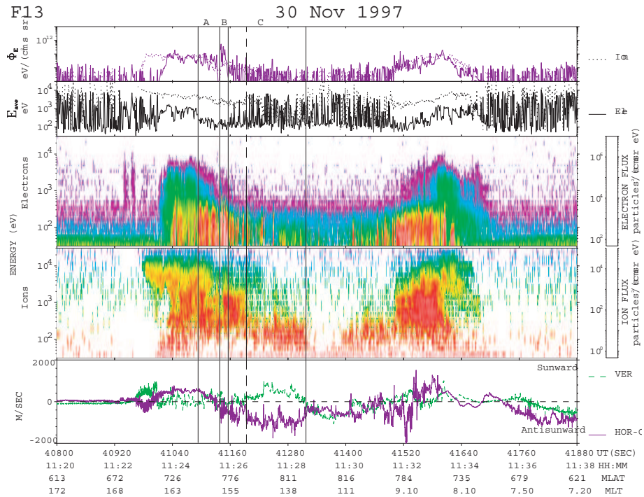
Fig. 5. DMSF F13 particle precipitation and ion drift data for the interval 11:20–11:38 UT. Panels from top to bottom show: (i) energy flux for electrons and ions (dotted), (ii) average energy of electrons and ions (dotted), (iii) electron and (iv) ion differential fluxes (color-coded according to scale to the right), and (v) horizontally across-track (violet) and vertical (green) ionospheric ion drift components. Different latitude regimes of discrete auroral precipitation on the dusk side are marked by vertical guidelines.
