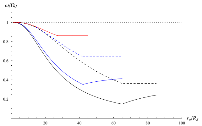
Fig. 11. Normalised plasma angular velocity profiles plotted versus equatorial radial distance for the case of an expansion of the magnetopause due to a sudden fall in solar wind dynamic pressure. The red solid line shows the initial steady state with a magnetopause at 45 R_J . The blue and black solid lines then show the transient profiles following an outward expansion of the magnetopause to 65 and 85 R_J , respectively. The blue and black dashed lines show the steady states to which these profiles relax after a \sim 1 – 2 day interval. The horizontal dotted line shows the condition of rigid plasma corotation.
