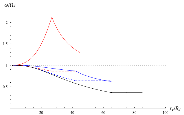
Fig. 5. Plots of the normalised plasma angular velocity shown versus equatorial radial distance for the case of solar wind compression of the magnetosphere. The black solid line shows the initial steady state profile with a magnetopause at 85 R_J and a boundary between the middle and outer magnetosphere at 65 R_J (the “baseline” model). The blue and red solid lines then show the transient profiles following a rapid inward compression of the magnetopause to 65 and 45 R_J , respectively. The red and blue dashed lines show the steady states to which these profiles relax after a \sim 1 – 2 day interval. The horizontal dotted line corresponds to rigid plasma corotation with the planet.
