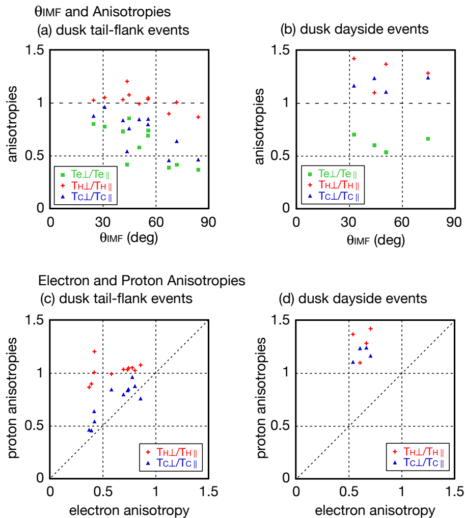
Fig. 10. Statistical plots of observed temperature anisotropies. The top two panels show the dependence of the anisotropies on the IMF latitudinal angle ( \theta_{IMF} ) for (a) tail-flank events and (b) dayside events. The bottom two panels present the relation between electron anisotropy and proton anisotropies for (c) the tail-flank and (d) the dayside events. Green squares, blue triangles, and red plus symbols correspond to the anisotropies of the electrons, the cold proton component, and the hot proton component, respectively.
