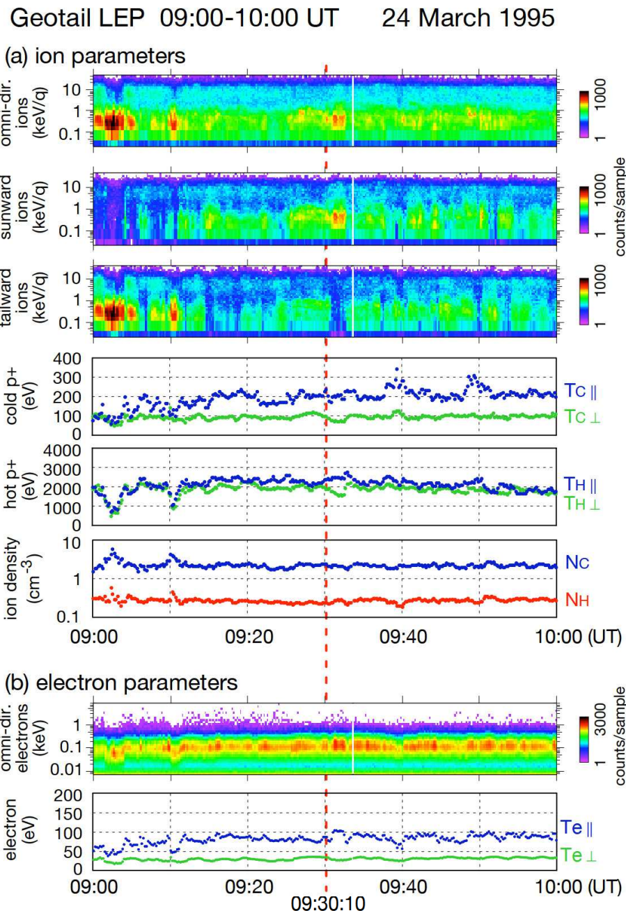
Fig. 1. Geotail observations between 09:00–10:00 UT on 24 March 1995. Panel (a) shows the ion observations. From the top, E-t spectrograms of omni-directional, sunward, and tailward ions, temperatures and densities of cold and hot proton components are presented. The perpendicular (parallel) temperature is shown by the green (blue) points, the density of the cold (hot) component is shown by the blue (red) points. Panel (b) shows the electron observations. E-t spectrogram of omni-directional electrons (7.4 eV–8.5 keV) and their temperatures are shown.
