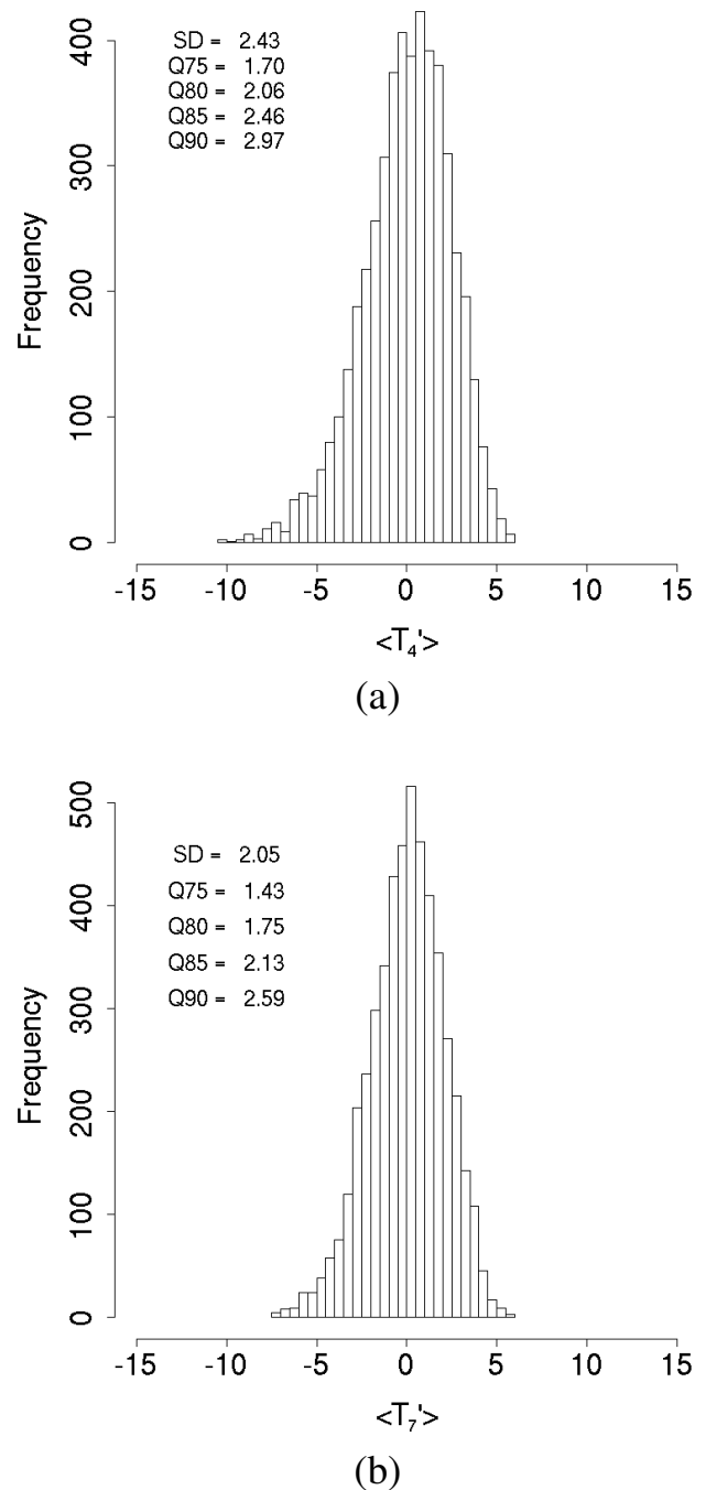
Fig. 2. Frequency distributions of the mean temperature anomalies over the target area (a) 4-day averaged anomaly and (b) weekly averaged anomaly. SD is standard deviation. Q75, Q80, Q85, Q90 are the percentile values at 75%, 80%, 85%, and 90% level. ( ^\circ C).
