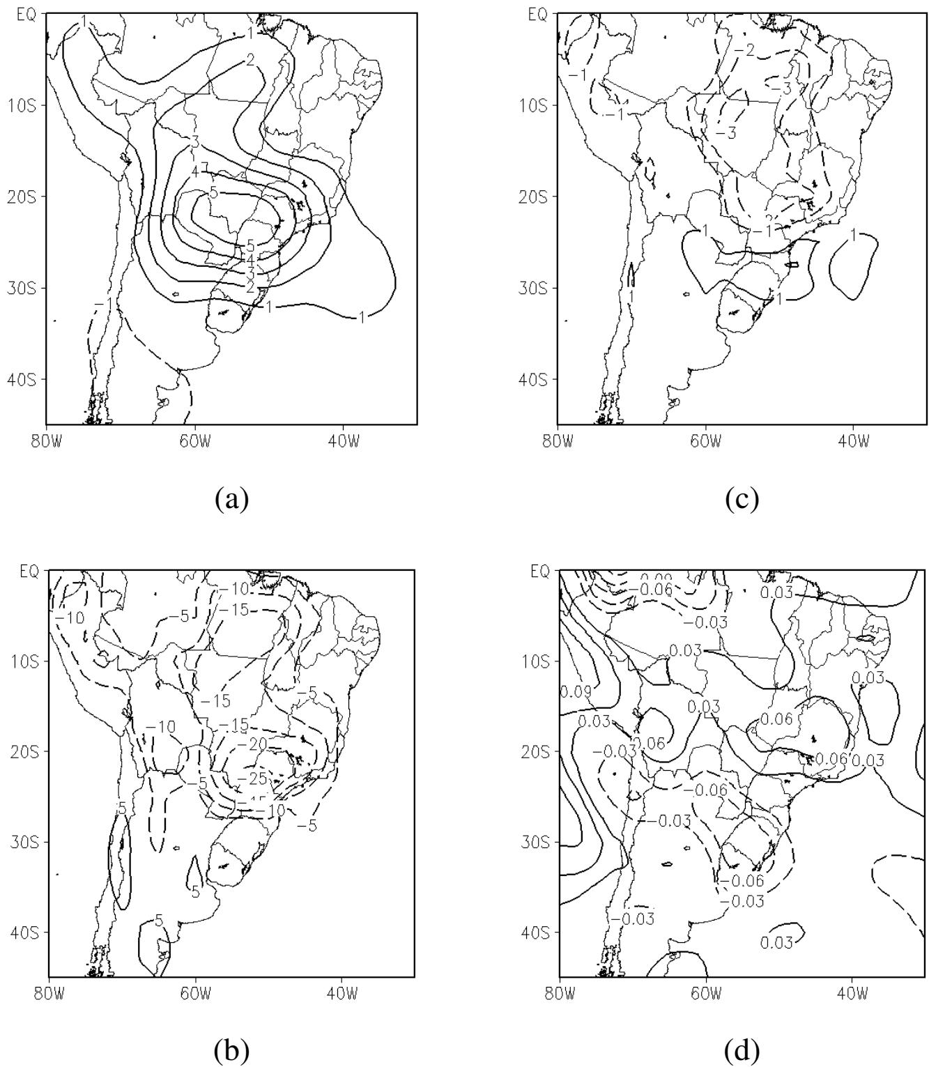
Fig. 5. Composite mean (a) surface temperature anomaly (°C), (b) specific humidity anomaly (g/kg), (c) relative humidity anomaly (%), and (d) 500-hPa \omega ( \text{Pa s}^{-1} ) for 17 strong WDSs during 1961–2003.
