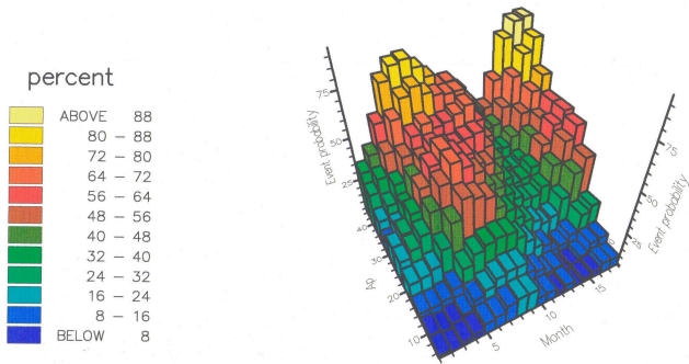
Fig. 3. Probability of at least one absorption event occurring per day at South Pole as functions of month and A_p . The first six months are repeated after month 12 (December).
