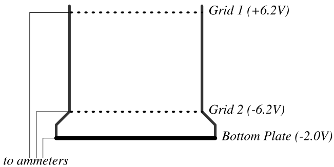
Fig. 1. The principle of the DUSTY probe, with its grid 1 to close the interior for ambient plasma, grid 2 to detect the effect of secondary charge production, and the bottom plate which will mainly detect directly impacting charged dust particles.
