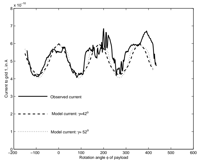
Fig. 11. Model calculations fitted to currents measured by grid 1 in the upper part of the dust cloud between heights 83.38 and 83.63 km. As for Fig. 10 we have made models for two coning angles. We have for these cases not included any production of positively charged fragments; see discussion in text. For \gamma=42^\circ the model parameters are \eta_S=100 , b=1.2 and the secondary production curve [30, 55, 75]. For \gamma=52^\circ we used \eta_S=80 , b=1.0 and a secondary production curve [30, 70, 80].
