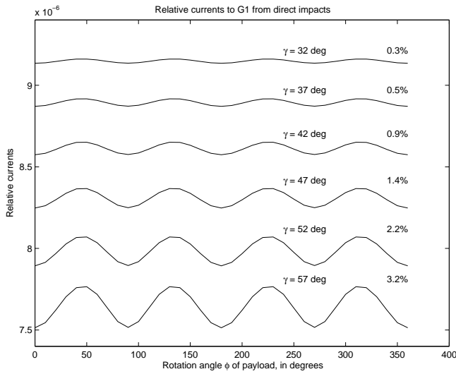
Fig. 7. Examples of how the currents to grid 1 would appear for a constant flux of charged particles onto the grid, without any effects of secondary currents due to charged fragment production. We show the resulting currents for several coning angles of the payload. The frequency of the modulation is clearly 4 times the payload spin rate and the modulation is very small, of the order of 1% only.
