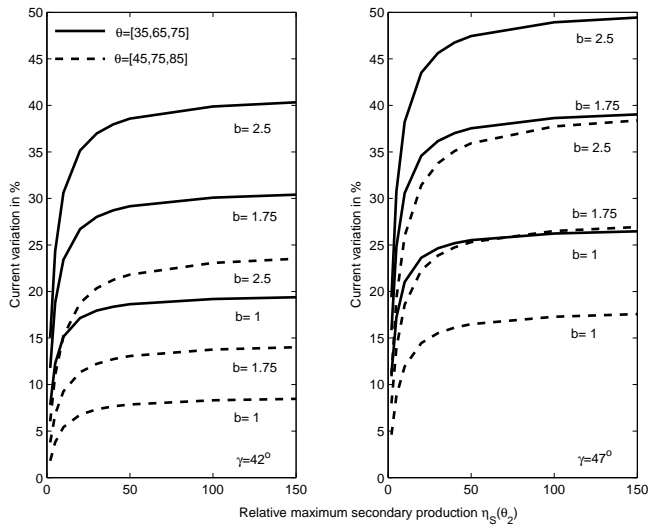
Fig. 9. The dependence of the current modulation on the maximum secondary production, for a different choice of coning angle, focusing on parameter and secondary production curves. The chosen parameters are given in the figures.
