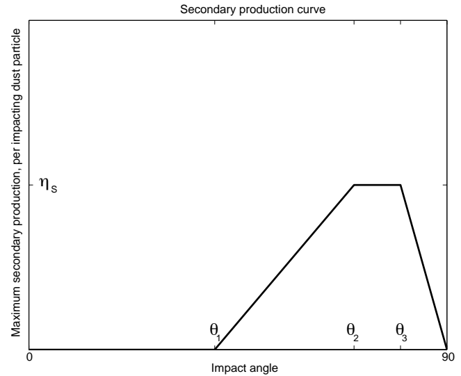
Fig. 6. The impact angle dependence for charged fragment production. The production of secondary fragments starts at impact angle \theta_1 , peaks in the interval between \theta_2 and \theta_3 and goes to zero at 90^\circ impact angle.
