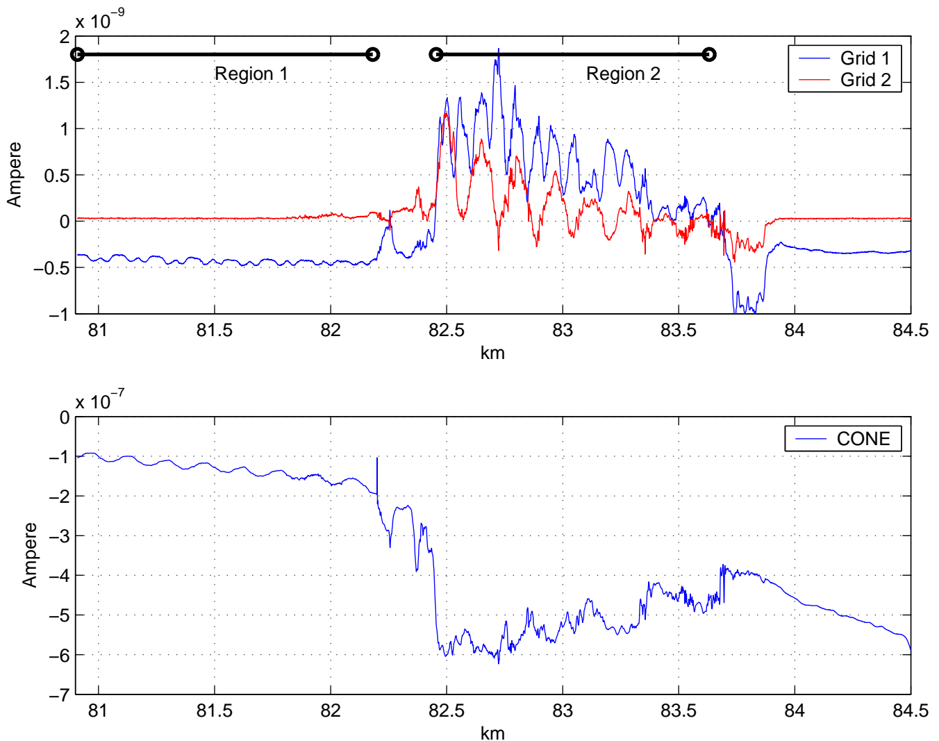
Fig. 4. The currents to grid 1 and grid 2, as measured by the DUSTY probe, and the electron current measured by the CONE probe, all on the flight ECT-07 (DUSTY 2).
