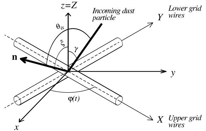
Fig. A1. The coordinate system used to describe the coordinate system of the rotating grid 1 wires and the geometry of impacts. For details see text.
