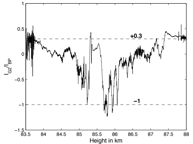
Fig. 3. The figure shows the ratio between the current to grid 2 and the bottom plate. The limit 0.3 is from Eq. (4) when secondary production is negligible while -1 is when it is dominant.
