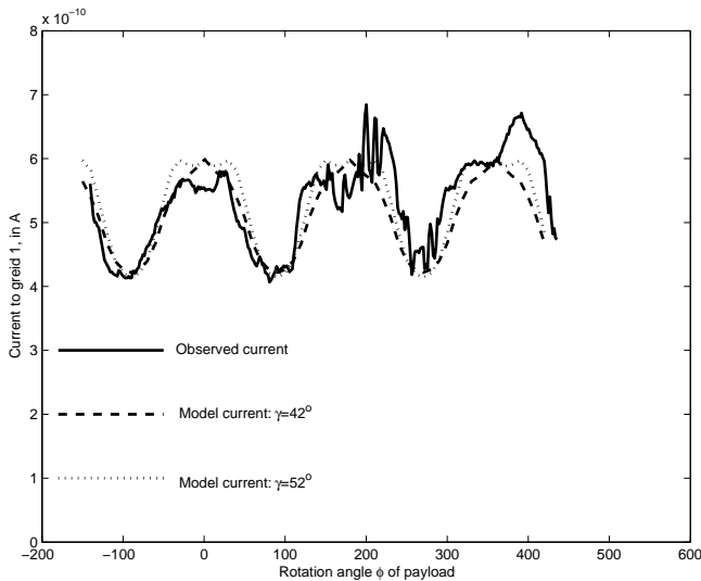
Fig. 12. Models for the same height interval as in Fig. 11, but in this case the secondary production curve has been chosen as [20, 80, 85] for both coning angles to investigate the consequence of a more extreme production. There is no production of positively charged fragments. The other parameters are for \gamma=42^\circ , chosen as \eta_S=60 and b=1.4 and for \gamma=52^\circ , \eta_S=60 and b=1 .
