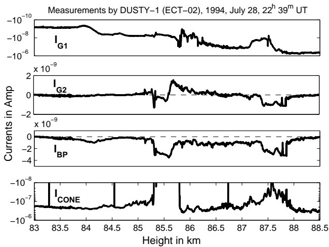
Fig. 2. Four currents measured by the rocket flight ECT-02 on up-leg. From top panel and down: Current to grid 1, grid 2 and the bottom plate in the DUSTY probe in front of the payload. The electron current measured by the CONE instrument, at the rear of the payload.
