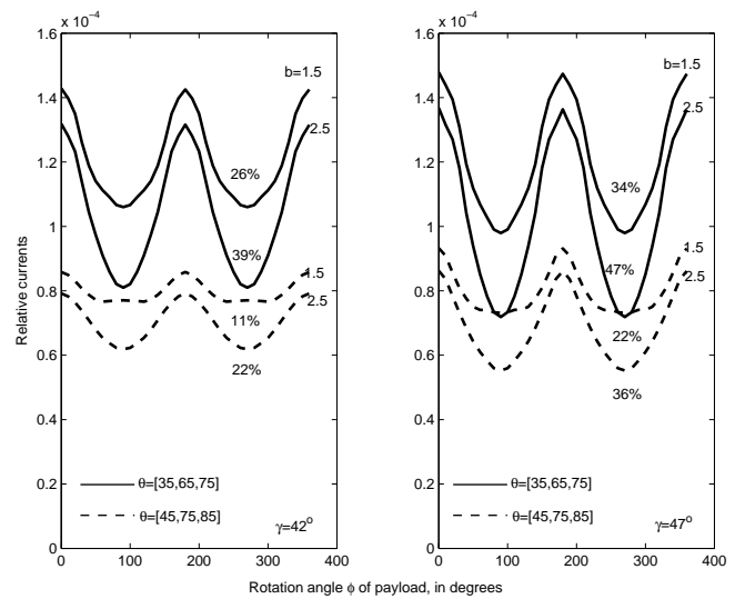
Fig. 8. Some examples where the secondary production and re-absorption of fragments are included. Only negatively charged fragments are produced, with a maximum secondary production \eta_S = 50 . The results are for two coning angles \gamma , for two values of the focusing parameter b and two different secondary production curves [\theta_1, \theta_2, \theta_3] . The chosen parameters are given in the figures. The frequency of the modulation is now 2 times the payload spin rate with a considerable modulation.
