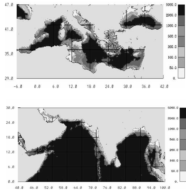
Fig. 1. Mediterranean Sea and Indian Ocean bathymetry (m).
