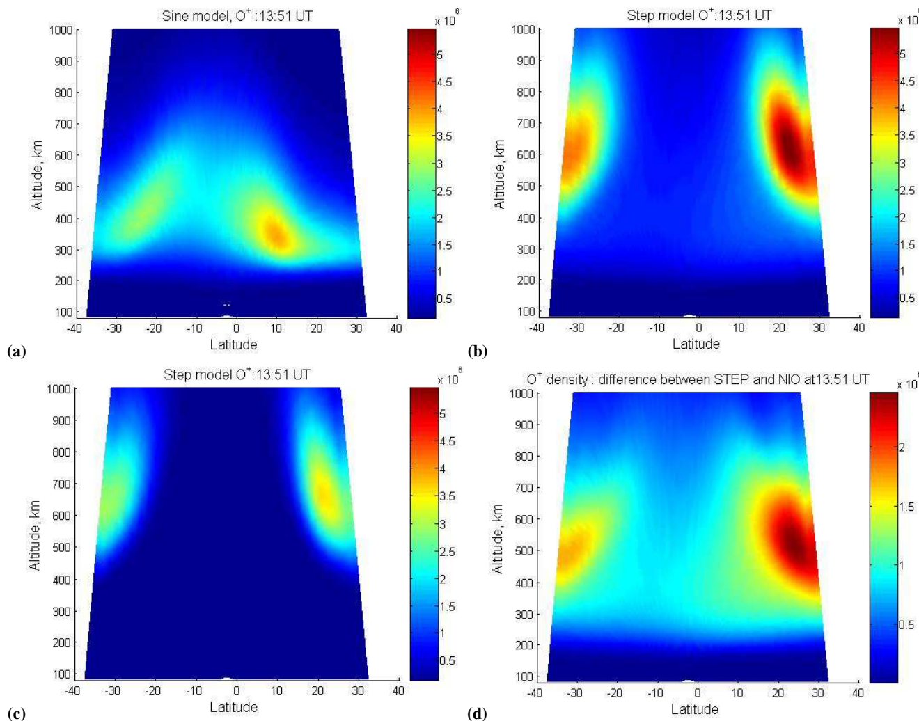
Fig. 1. Modeling of O + ion uplift during strong IEF events/magnetic storms. The color insets on the right of each panel show the local ion density in cm -3 . The following models of E \times B drift were used: a “sine” wave background model (a), a PPEF step model (b), and the step model without solar photoionization (c). All density profiles are shown for ~02:00 p.m. local time. Differences in the ion density between the step model with and without ionization is also shown (d). Notice the maximum difference occurs at ~500 km and for ~25° latitude.
