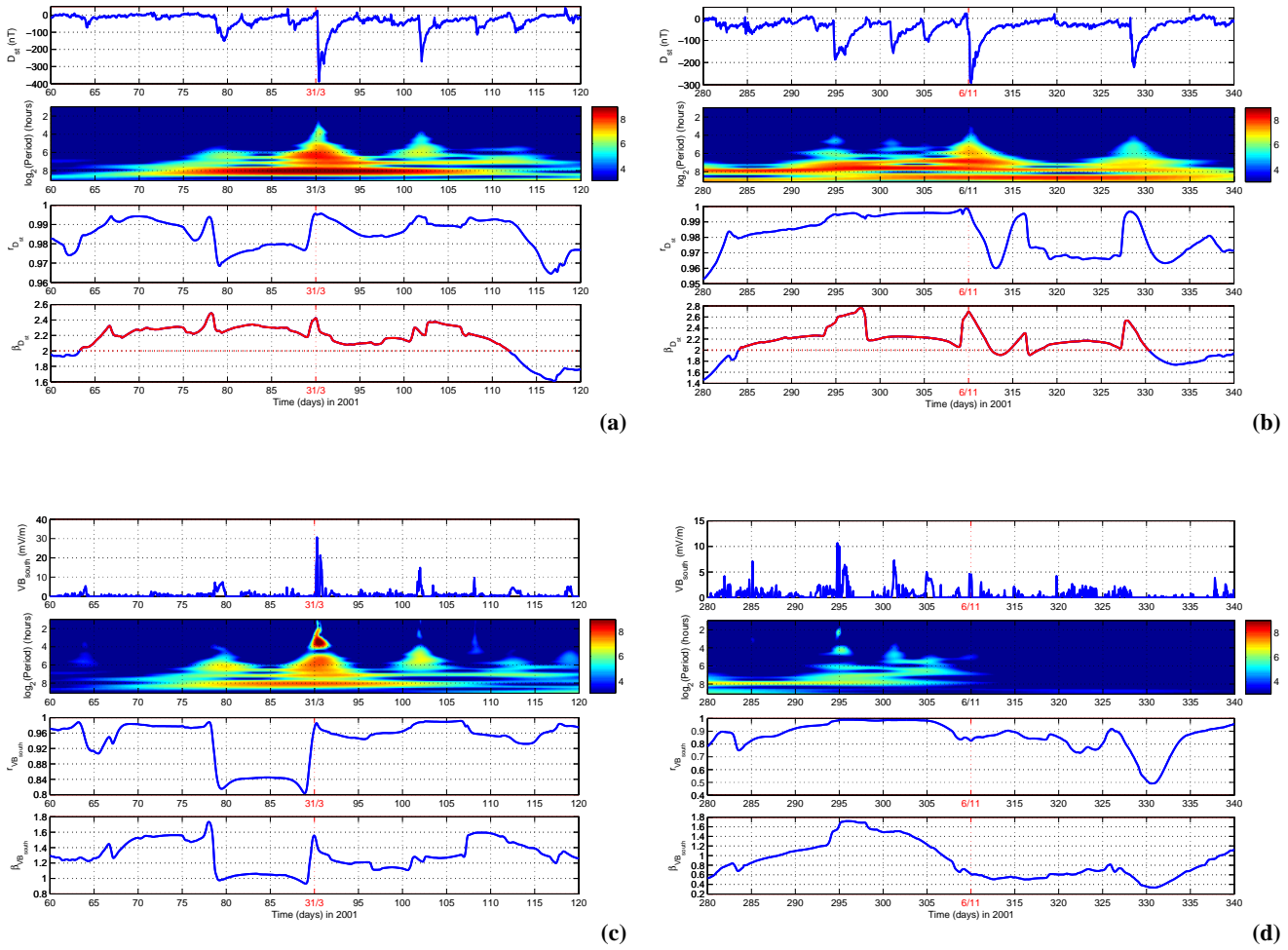
Fig. 4. (a)–(d) A close-up on days 60 to 120 and 280 to 340 of Figs. 1–2. At each subfigure: D_{ST} or VB_{South} time series and its wavelet power spectrum (upper panels), corresponding linear correlation coefficients r and spectral exponents \beta (lower panels).
