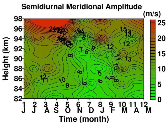
Fig. 12. Same as Fig. 9 but for meridional semidiurnal tide.
