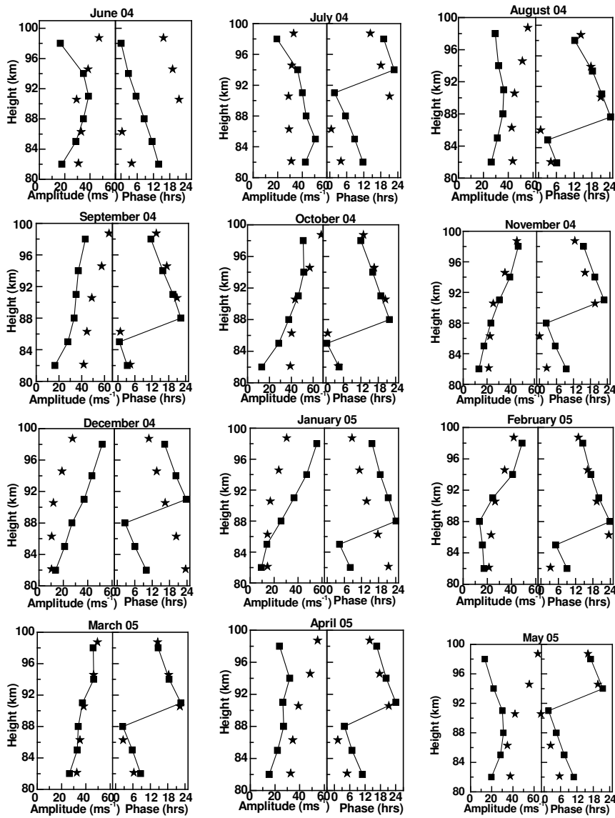
Fig. 4. Same as Fig. 3, but for meridional diurnal tides.
