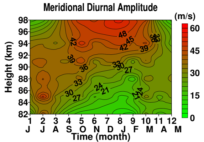
Fig. 10. Same as Fig. 9 but for meridional diurnal tide.
