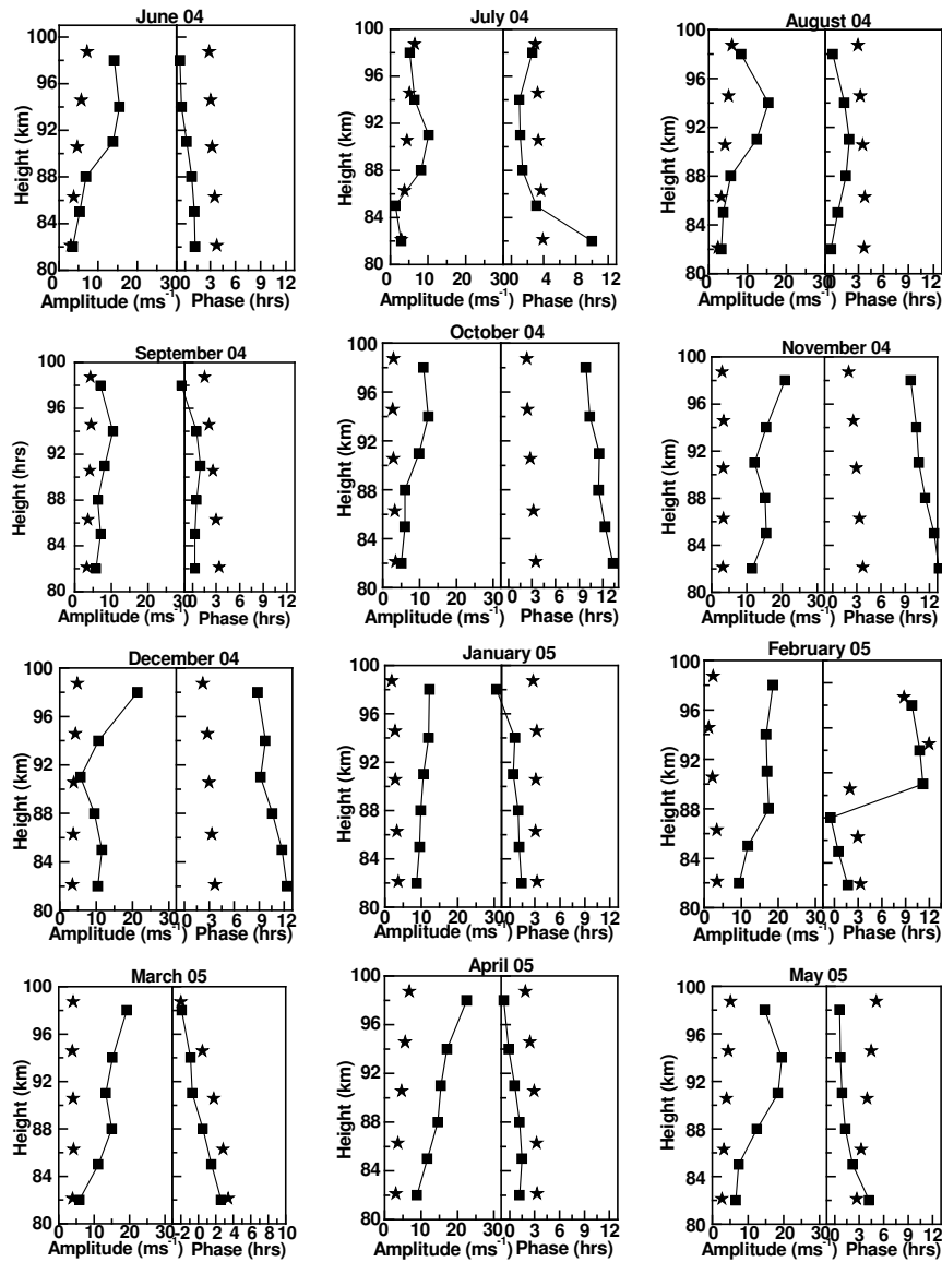
Fig. 5. Same as Fig. 3, but for zonal semidiurnal tides.
