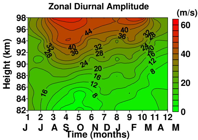
Fig. 9. Time-height contours of zonal diurnal amplitude showing the seasonal variation starting from June 2004 to May 2005. Contour intervals are 4 \text{ ms}^{-1} .
