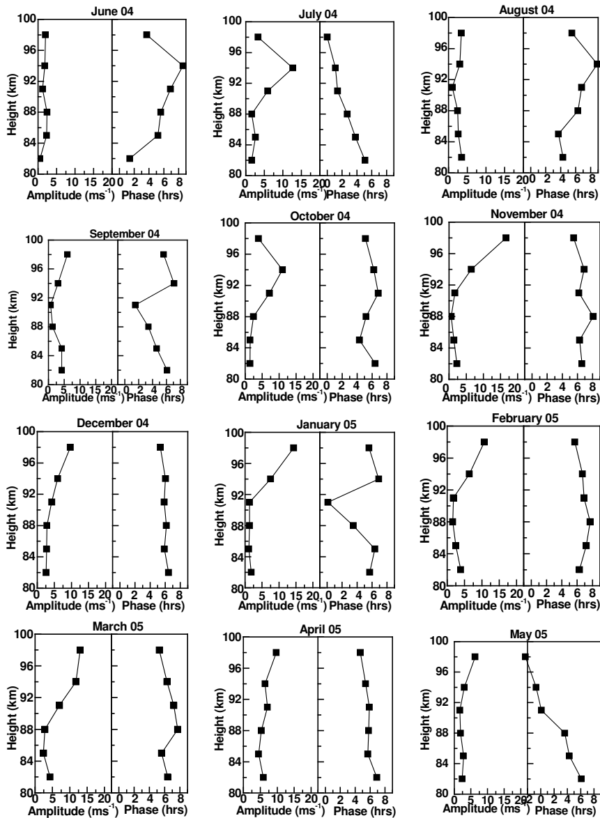
Fig. 8. Same as Fig. 3, but for meridional terdiurnal tides.
