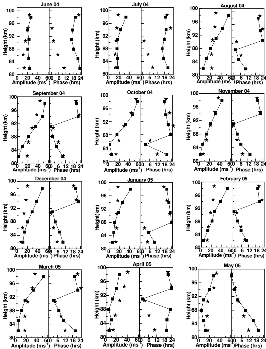
Fig. 3. Height profile of amplitude and phase of zonal diurnal tides from June 2004 to May 2005. Squares represent the observed values and stars represent the GSWM02 model values.
