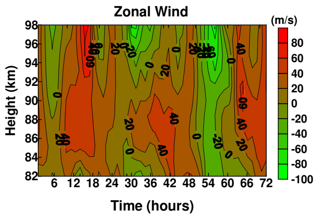
Fig. 1. Time-height contour of the zonal wind observed during three consecutive days (72 h). Red contours represent the westerly winds and green the easterly winds.
