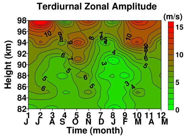
Fig. 13. Same as Fig. 9 but for zonal terdiurnal tide.
