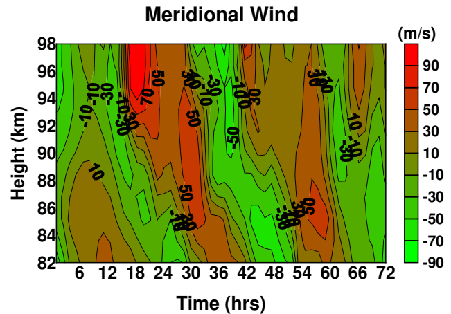
Fig. 2. Time-height contour of the meridional wind observed during three consecutive days (72 h). Red contours represent the southerly winds and green the northerly winds.
