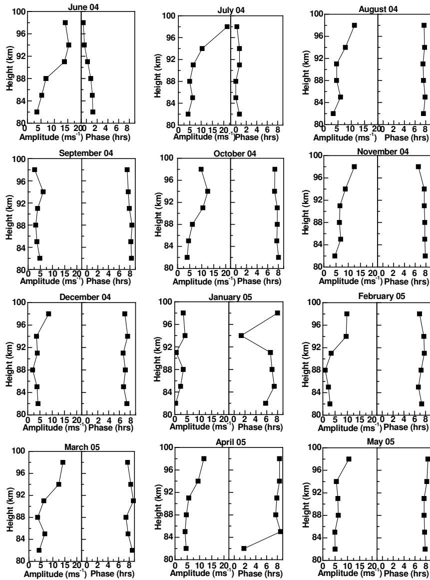
Fig. 7. Same as Fig. 3, but for zonal terdiurnal tides.
