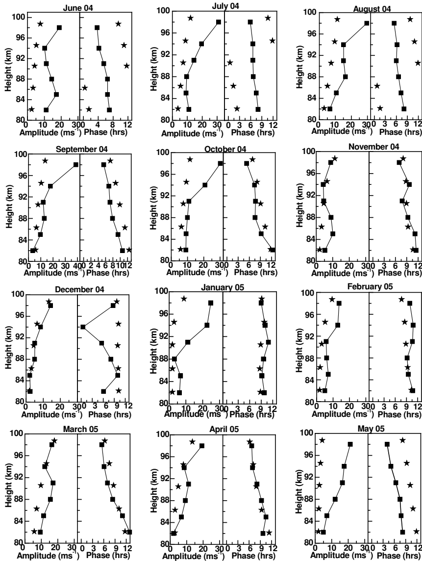
Fig. 6. Same as Fig. 3, but for meridional semidiurnal tides.
