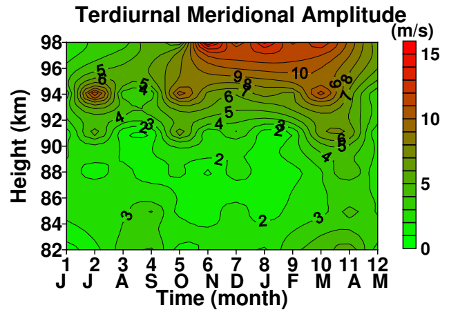
Fig. 14. Same as Fig. 9 but for meridional terdiurnal tide.
