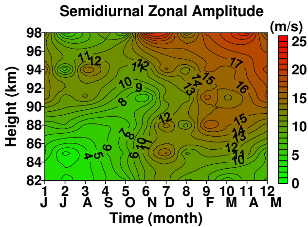
Fig. 11. Same as Fig. 9 but for zonal semidiurnal tide.
