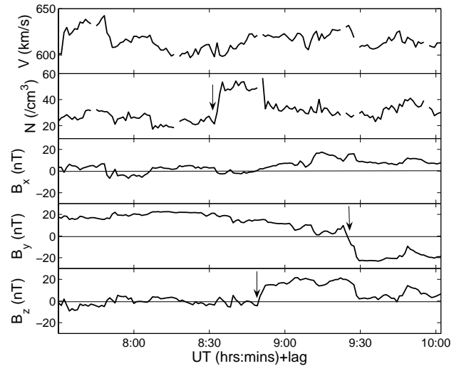
Fig. 7. Data from the ACE satellite for 27 November, 2000, lagged by 41 min. Arrows mark the times of significant changes that result in observed effects in the ionosphere.
