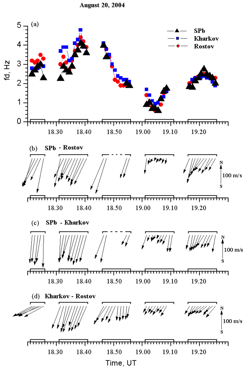
Fig. 10. Median values of Doppler frequency shifts averaged on the 1-min interval for the HF diagnostic signals scattered from AFAs on the Armavir–Sura–St. Petersburg, Serpukhov–Sura–Kharkov, and Serpukhov (Moscow)–Sura–Rostov paths in the course of the Sura heating experiment on 20 August 2004 (a); simulated vectors of TID phase velocities for the same event using the pair of paths with reception points at St. Petersburg and Rostov (b); the same as in (b) but for St. Petersburg and Kharkov pair paths (c); the same as in (b) and (c) but for Kharkov and Rostov pair paths (d).
