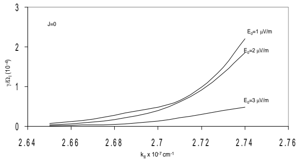
Fig. 4. Variation of growth rate ( \gamma / \Omega_i ) versus wave vector k_{||} \text{cm}^{-1} for different values of parallel electric field E_0 , and distribution index J=0 .
