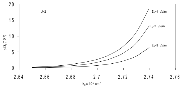
Fig. 6. Variation of growth rate ( \gamma / \Omega_i ) versus wave vector k_{||} \text{cm}^{-1} for different values of parallel electric field E_0 , and distribution index J=2 .
