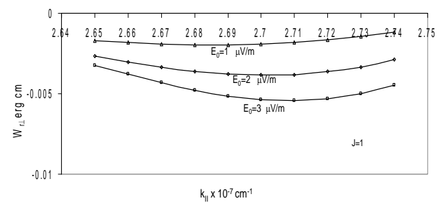
Fig. 8. Variation of perpendicular resonant energy W_{r\perp} erg cm versus wave vector k_{||} \text{cm}^{-1} for different values of parallel electric field E_0 , and distribution index J=1 .
