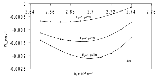
Fig. 7. Variation of perpendicular resonant energy W_{r\perp} erg cm versus wave vector k_{||} \text{cm}^{-1} for different values of parallel electric field E_0 , and distribution index J=0 .
