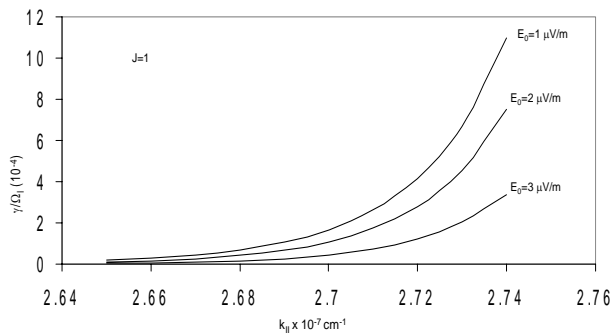
Fig. 5. Variation of growth rate ( \gamma / \Omega_i ) versus wave vector k_{||} \text{cm}^{-1} for different values of parallel electric field E_0 , and distribution index J=1 .
