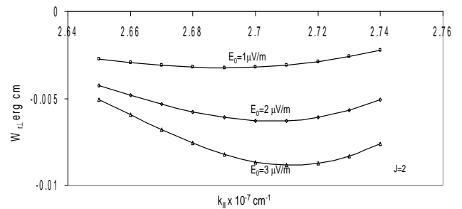
Fig. 9. Variation of perpendicular resonant energy W_{r\perp} erg cm versus wave vector k_{||} \text{cm}^{-1} for different values of parallel electric field E_0 , and distribution index J=2 .
