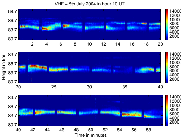
Fig. 7. One hour of raw data. The heater transmitter is now run at full power in all cycles. The overshoot cycles are each 3 m long and the heater is on for 20 s. This is clearly shown as a reduced intensity with 3 m interval, lasting for 20 s, followed in most cases by strong overshoots.
