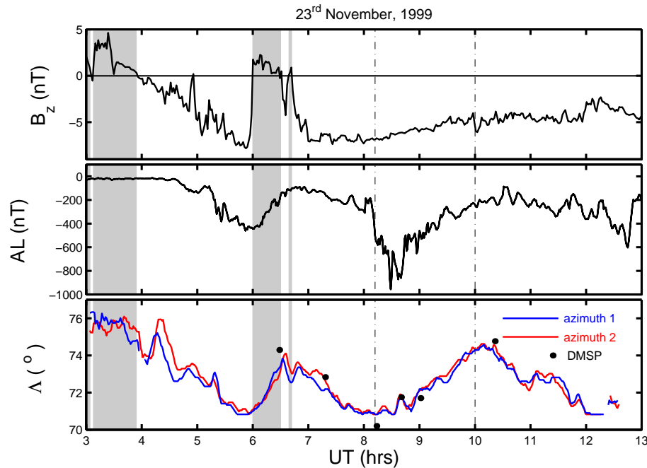
Fig. 3. (Top) The B_Z component of the IMF in the GSM coordinate system, observed by the WIND spacecraft, lagged by the predicted propagation time from the satellite to the dayside magnetopause. (Middle) The auroral AL index. (Bottom) The latitude of the polar cap boundary determined from (in blue) beam 1 (azimuth 344^\circ E of N, along the geomagnetic meridian) and (in red) beam 2 (azimuth 359^\circ E of N, along the geographic meridian) of the EISCAT VHF radar operated in the CP-4-B mode (as shown in Fig. 2). The black points are the open closed boundary intersections seen by DMSP satellites at an MLT within 1.5 h of that of beam 1 of the EISCAT radar. The areas shaded grey are northward IMF and the vertical dot-dashed lines mark the expansion/recovery phases of the larger substorm.
