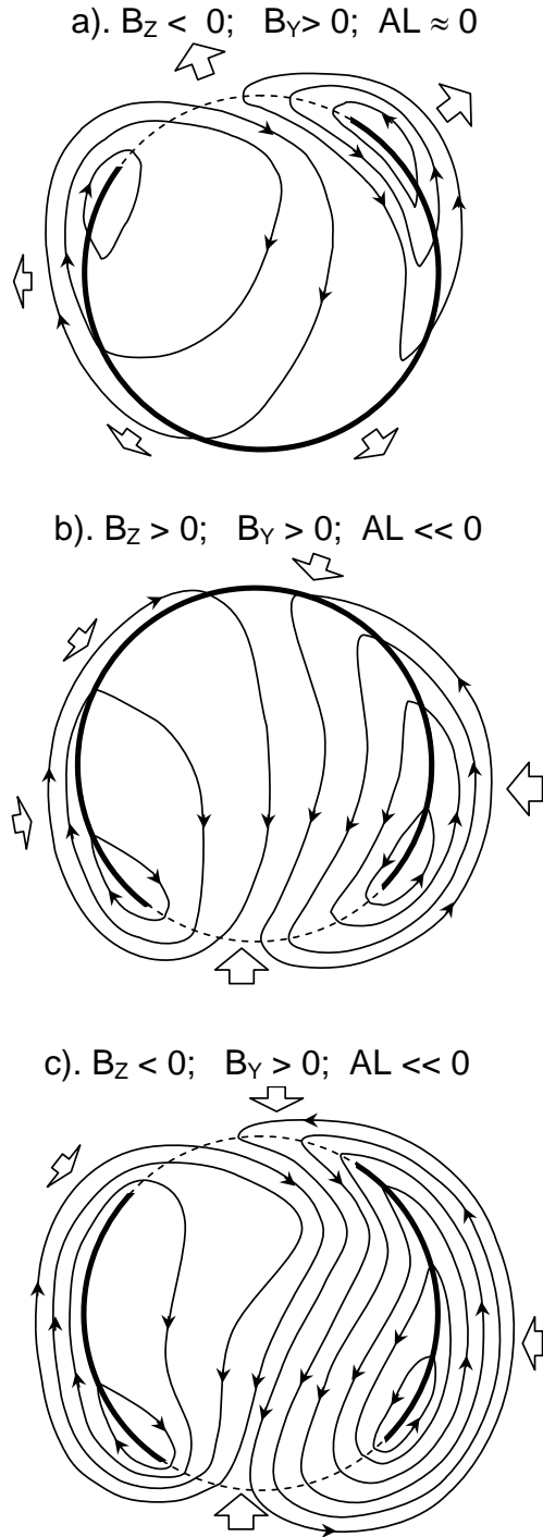
Fig. 4. Schematic of polar cap expansions and contractions. Lines with arrows are flow streamlines, thick solid lines are adiarocic (non-reconnecting) open closed field line boundary and dashed lines are footprints of the active dayside and nightside reconnection sites (in the magnetopause and cross-tail current sheet, respectively). Open arrows show the motion of the open-closed boundary. (a) Growth phase with IMF B_z < 0 , B_y > 0 , and AL \approx 0 . (b) Expansion-recovery phase with northward IMF: B_z > 0 , B_y > 0 , AL \ll 0 . (c) Expansion-recovery phase with southward IMF: B_z < 0 , B_y > 0 , AL \ll 0 .
