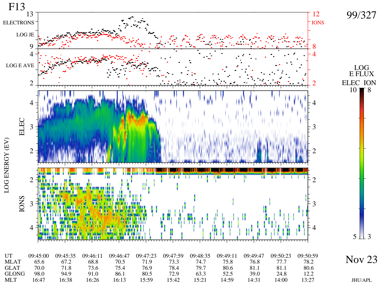
Fig. 7. Same as Fig. 5, showing a dusk pass of DMSP-F13 through the footprint of an adiaric (non-reconnecting) open-closed boundary near 16:00 MLT. Note that no sheath-like precipitation was observed.
