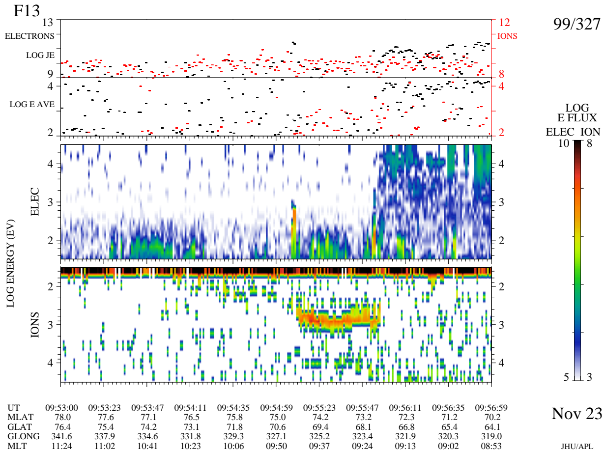
Fig. 8. Same as Fig. 5, showing a dawn pass of DMSF-F13 through the footprint of an adiaroc (non-reconnecting) open-closed boundary near 09:00 MLT. Note that sheath-like precipitation was observed, but ion energies near the open-closed boundary did not exceed 1 keV.
