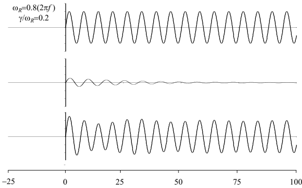
Fig. 12. Top panel: Directly driven reflected signal when \omega_R=1.6\pi f . Middle panel: Contribution from excited leaky waveguide mode. Bottom panel: Superposition.
