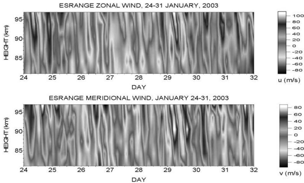
Fig. 5. Contour plot of the zonal and meridional winds measured by the Esrangle meteor radar from 24 January to 1 February. A strong semi-diurnal tide was present during the campaign.
