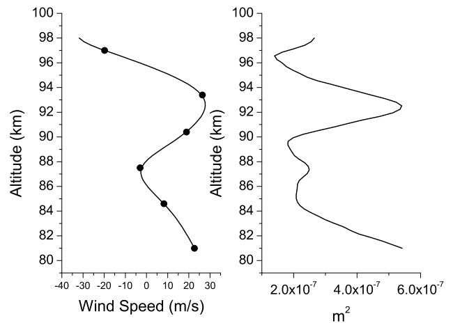
Fig. 16. Left plot shows the vertical wind profile (Esrangle radar data) in the direction of wave 1 observed on 27/28 January at 16:00 UT. The sign indicates the direction of the wind relative to the wave motion (positive in same direction). Right plot shows the squared value of the vertical wavenumber as a function of height. The positive value for m^2 throughout the emission layer heights is indicative of a freely propagating wave.
