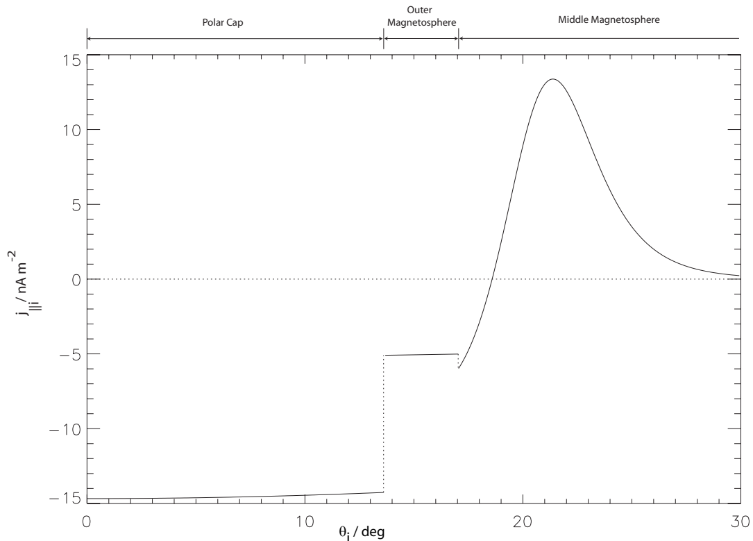
Fig. 6. Plot of the distributed field-aligned current density j_{\parallel i} obtained from Eq. (34) from the rotational flow component only, shown versus co-latitude \theta_1 . The horizontal bars at the top of the plot indicate the regions of co-latitude that map to the polar cap, the outer magnetosphere, and the middle magnetosphere regions. Positive values indicate currents directed upward out of the ionosphere, negative values indicate currents directed downward into the ionosphere, and the horizontal dotted line indicates the zero level.
