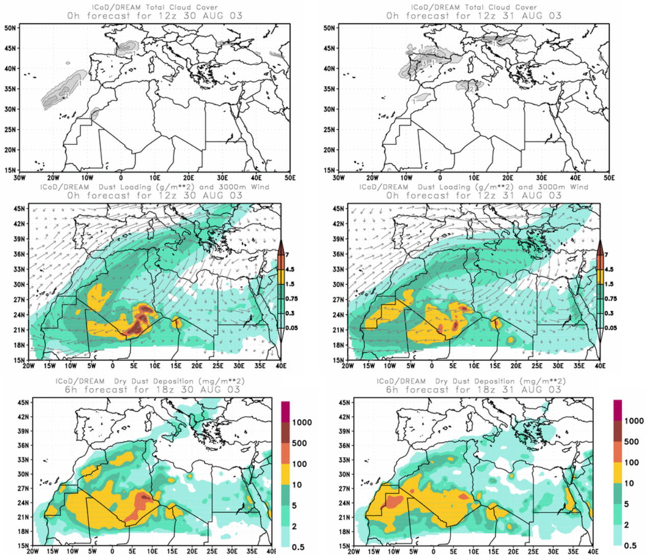
Fig. 6. Analysis of cloud cover and dust load (in \text{g}/\text{m}^2 ) for 30 and 31 August 2003 estimated by the DREAM model.
