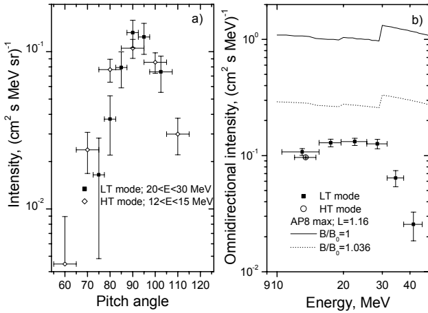
Fig. 4. (a) Equator pitch angle distributions of trapped protons at L=1.16 for different energy ranges (12–15 MeV–open rhombus, 20–30 MeV – solid squares). (b) Omnidirectional energy spectrum of trapped protons at L=1.16 measured in different NINA operational modes (HT– open circle; LT– solid squares); AP-8 MAX predictions for L=1.16 and for experimental B/B_0 range (solid line– B/B_0=1 ; dotted line– B/B_0=1.036 ).
