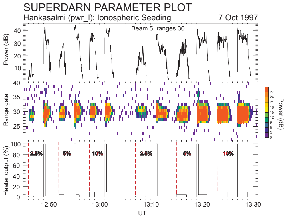
Fig. 8. The results of the ionospheric seeding experiment of 7 October 1997: The middle panel shows the backscatter power received by the Hankasalmi radar along beam 5 during heating with the Tromsø facility. Plotted in the upper panel is the backscatter power at range gate 30 along this beam. The lower panel depicts the heater output power throughout this interval.
