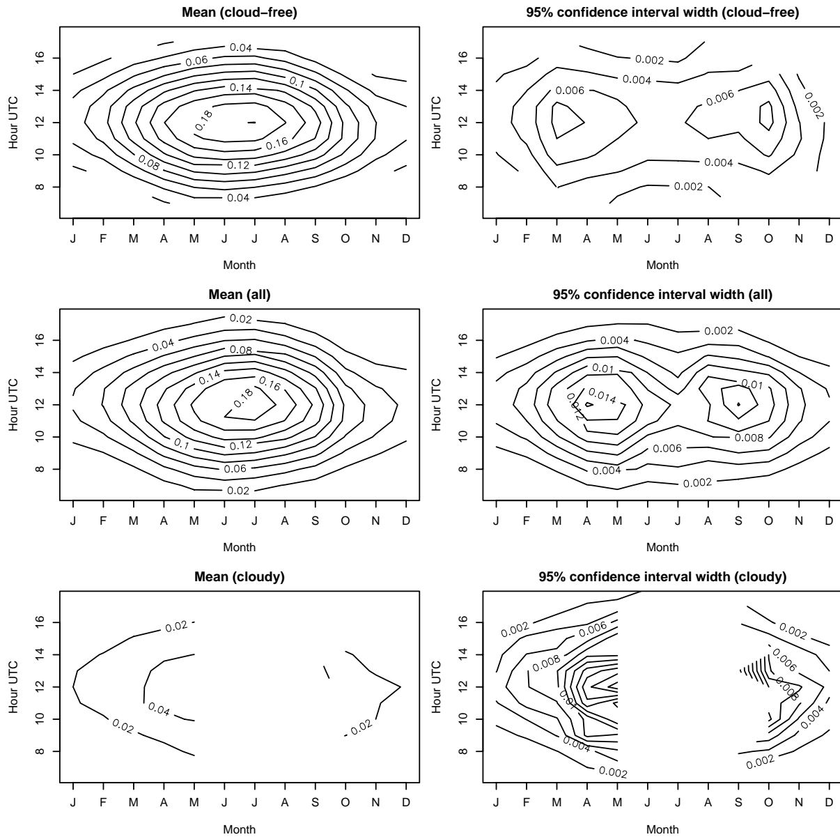
Fig. 11. Iso-irradiance lines of the mean of hourly ultraviolet erythemal irradiance (in Wm^{-2} ).
