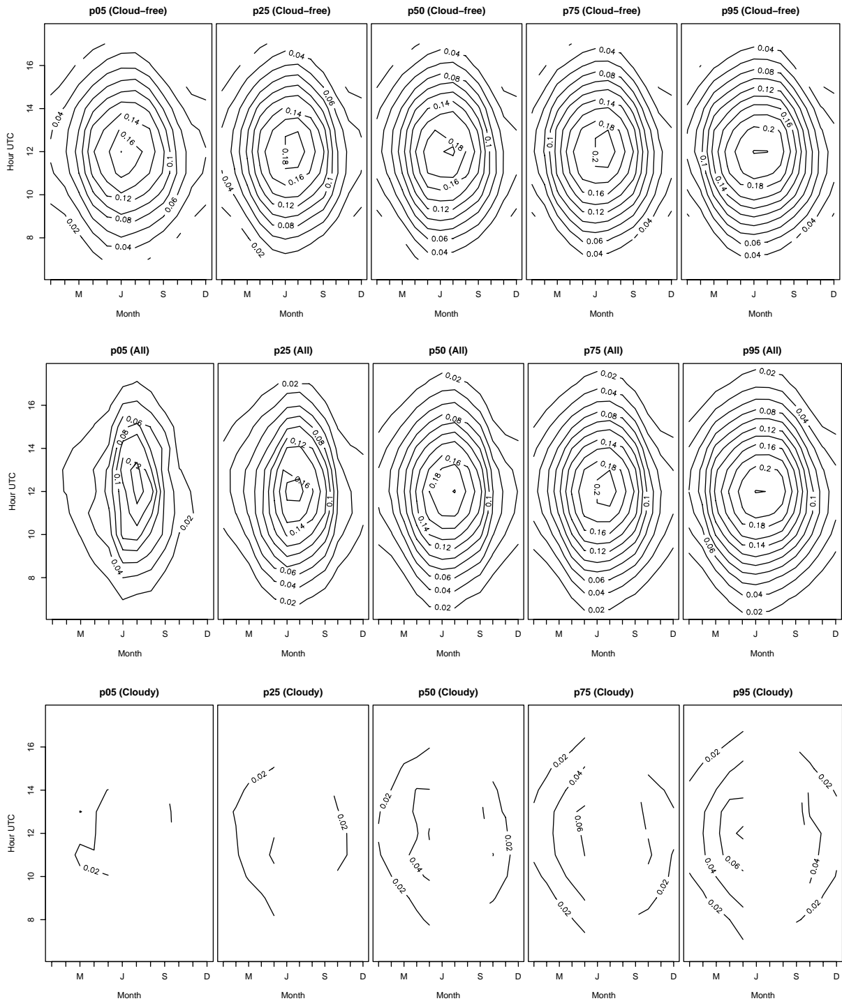
Fig. 10. Iso-irradiance lines of percentiles 5, 25, 50 (i.e. the median), 75 and 95 of hourly ultraviolet erythemal irradiance (in \text{Wm}^{-2} ) under cloud-free, all weather, and cloudy conditions.
