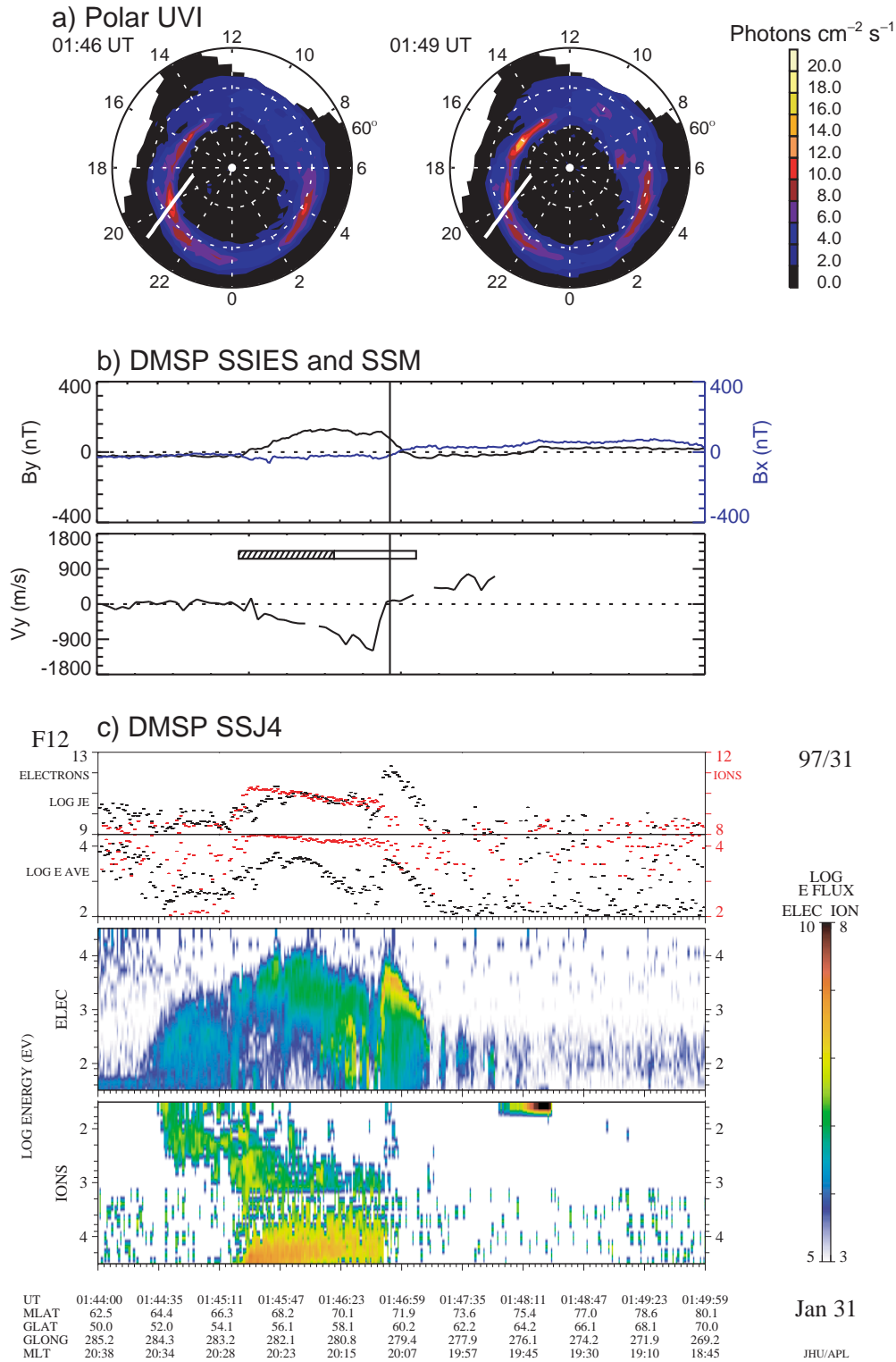
Fig. 2. A summary of observations for the 01:44–01:50 UT, 31 January 1997 event. (a) We selected two consecutive Polar UVI LBH-long auroral images which were closest to the period of the event. The white line on each image marks the trajectory of the DMSP F12 spacecraft, moving from the equator side of the aurora to the poleward side. The both ends of the line denote the locations of DMSP F12 spacecraft at the beginning and the end of the event. (b) The black (blue) curve in the magnetic field panel represents variations of the Y and X components of the magnetic field produced by field-aligned currents. The vertical line in the B_y/B_x and convection ( V_y ) panels denotes the location of the peak energy flux determined from (c) the DMSP electron energy flux data. The white (shaded) horizontal bar in the V_y panel represents the interval of large-scale region 1 (region 2) field-aligned currents. Note that the +X component is in the direction of the spacecraft velocity vector. The +Y component is perpendicular to the +X component and points toward the nightside of the orbit plane.
