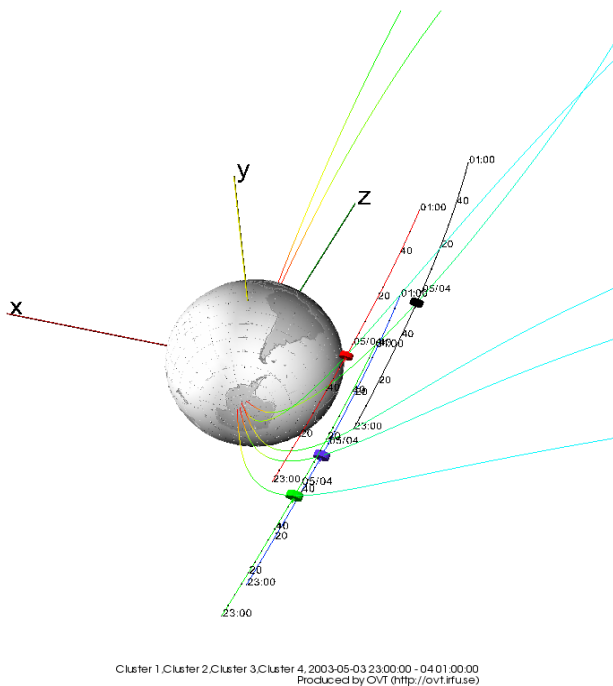
Fig. 10. Configuration of the Cluster spacecraft on 3 May, 23:00–4 May, 01:00 UT. Spacecraft 1 is represented by black, spacecraft 2 by red, spacecraft 3 by green and spacecraft 4 by blue color.
