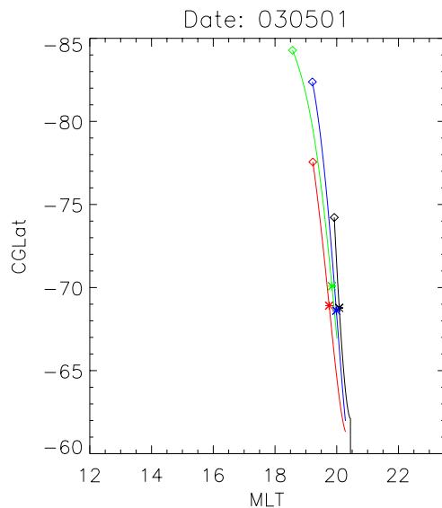
Fig. 9. Mapped location of the PS poleward boundary for Event 1 (asterisks). The color lines show the mapped orbit of the Cluster spacecraft. Black color corresponds to spacecraft 1, red to spacecraft 2, green to spacecraft 3 and blue to spacecraft 4. The diamonds mark the start point of each passage.
