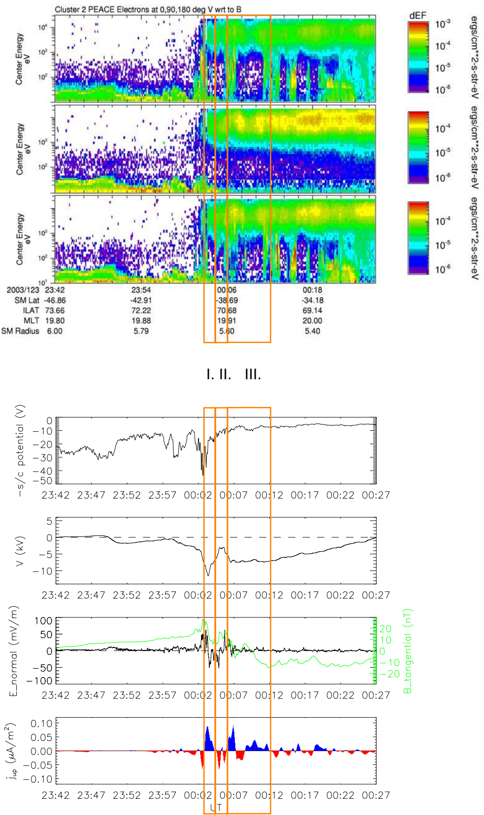
Fig. 17. Event 2 — data measured on board Cluster spacecraft 2. The description of the panels is the same as for Fig. 2.
