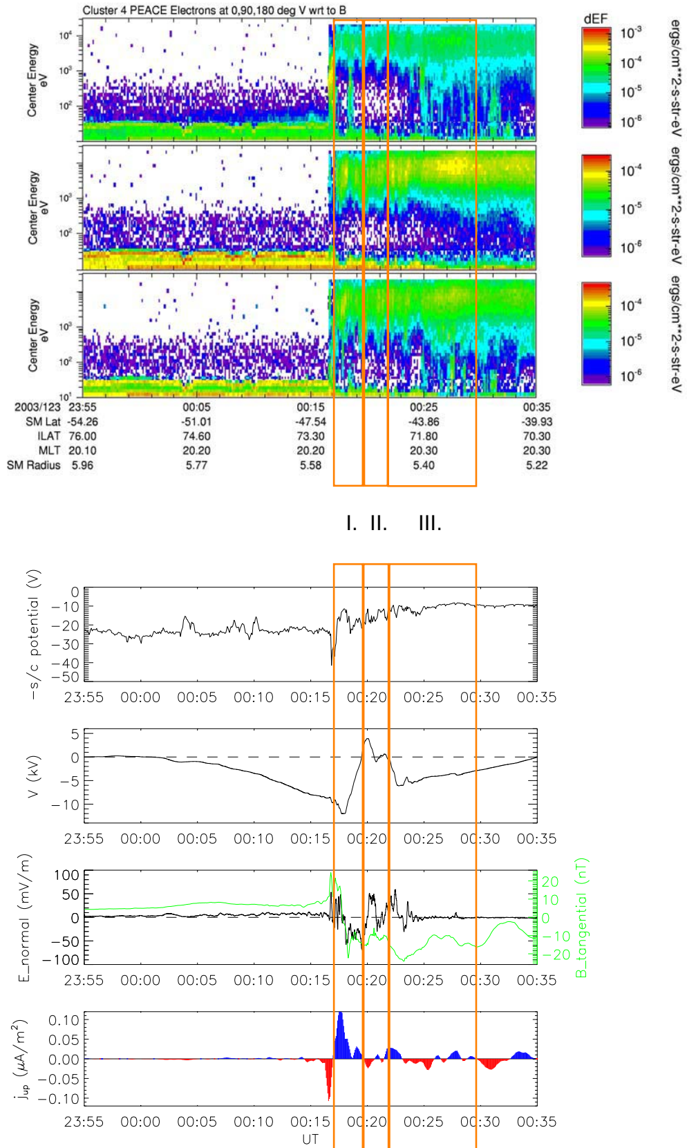
Fig. 18. Event 2 — data measured on board Cluster spacecraft 4. The description of the panels is the same as for Fig. 2.
