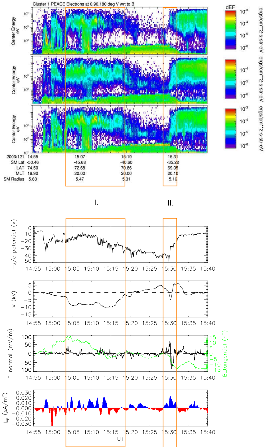
Fig. 2. Event 1 – 1 May 2003. Data measured on board Cluster spacecraft 1. Panels 1 to 3 – Electron energy flux spectrogram versus energy at pitch angles 0, 90 and 180°, respectively. Pitch angle of 0° corresponds to upgoing and 180° to downgoing electrons on the Southern Hemisphere. Panel 4 – Negative of the spacecraft potential. Panel 5 – Calculated perpendicular potential. Panel 6 – Electric field component normal to the structure and pointing equatorwards (black line); Magnetic field component tangential to the structure pointing eastwards (green line). Panel 7 – Field-aligned current density distribution, with blue color showing upflowing currents and red color downflowing currents.
