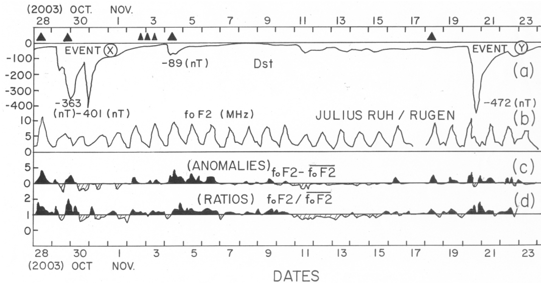
Fig. 1. Plots for the 27-d interval 28 October–23 November 2003 of the hourly values of (a) geomagnetic D_{st} , (b) ionospheric f_oF2 at the midlatitude European location Juliusruh/Rügen (54.6° N, 13.4° E), (c) f_oF2 anomalies, (d) f_oF2 ratios. Positive deviations and ratios above 1.0 are painted black, negative deviations and ratios below 1.0 are shown as hatched. The triangles indicate solar flare occurrences.
