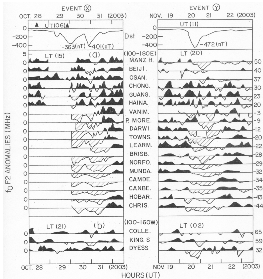
Fig. 3. Same as Fig. 2, for longitude belts (a) 100^{\circ} E– 180^{\circ} E, (b) 100^{\circ} W– 160^{\circ} W.
