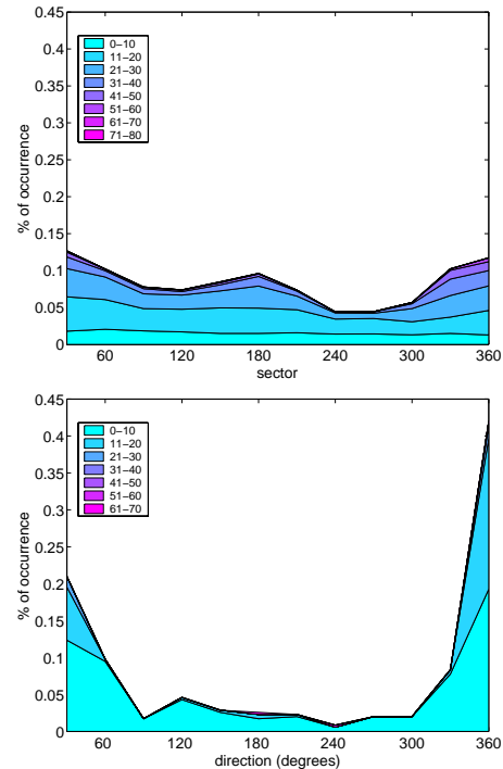
Fig. 13. Direction against percentage of occurrence for the current speed at location corresponding to VEINS FA/FB. Model (top) and observational (bottom) data are shown at about 300 m depth.
