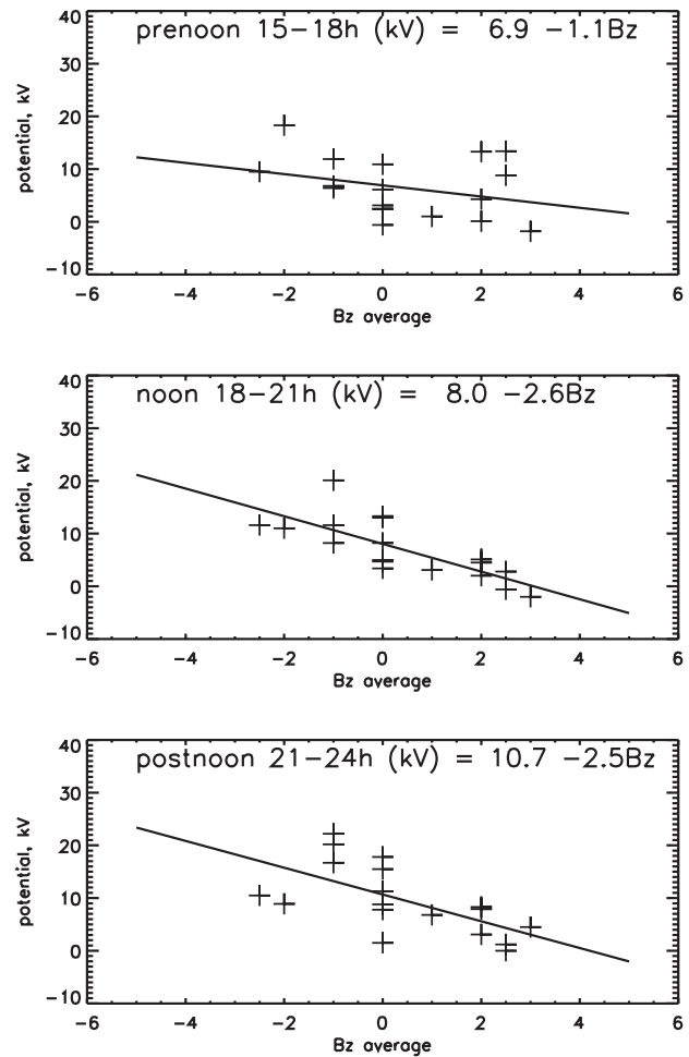
Fig. 4. Potentials calculated for three time intervals as a function of IMF B_z . The equations of the fitted lines are shown
