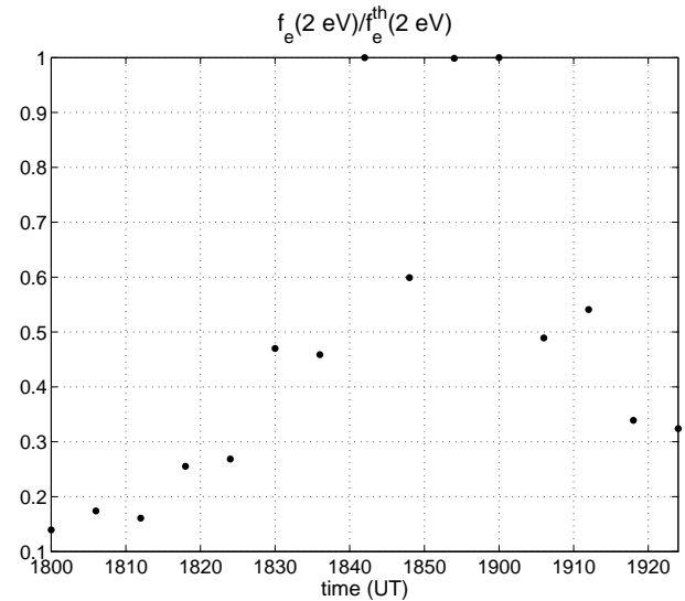
Fig. 8. Estimate of the ratio of f_e(E)/f_e^{th}(E) at 2 eV. Here f_e^{th}(E) denotes a thermal energy distribution. Note that the depletion is significant for the first five pulses when the approximate altitude of upper hybrid resonance is below 250 km and varies for the last pulses when the interaction altitude is above 250 km. This is consistent with the decrease in neutral concentrations with increasing altitudes.
