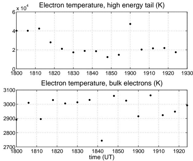
Fig. 7. Upper panel shows the electron temperature in the high energy tail, from 2 eV to approximately 20 eV. For comparison the lower panel displays the EISCAT UHF measurements of ( T_e ) at steady state in the region of highest temperature.
