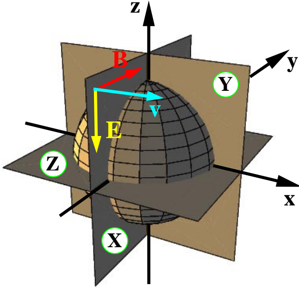
Fig. 3. Cross sections of the simulation box at the plane x=0 , y=0 and z=0 presented in Sect. 4.
