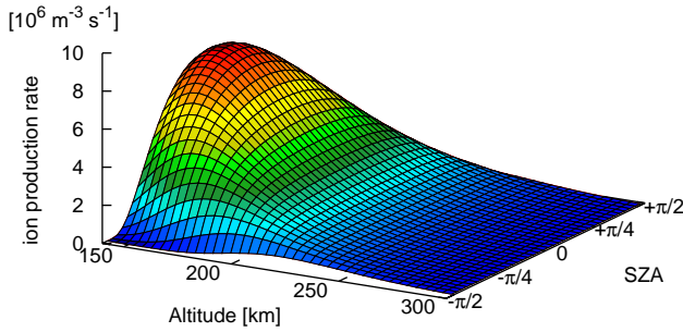
Fig. 6. Ion production rate of oxygen as a function of altitude and solar zenith angle (SZA) at solar minimum.
