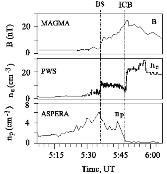
Fig. 2. Data obtained from different instruments on board Phobos-2 along an elliptical orbit from 8 February 1989 (adapted from Sauer and Dubinin, 2000). The ion composition boundary is recognized by a sharp increase in the electron density which indicates the ionospheric plasma and a decrease of the solar wind density. The magnetic field piled up until this position. The decrease of the proton density downstream of the BS probably results from a somewhat small angle of view of the ASPERA instrument.
