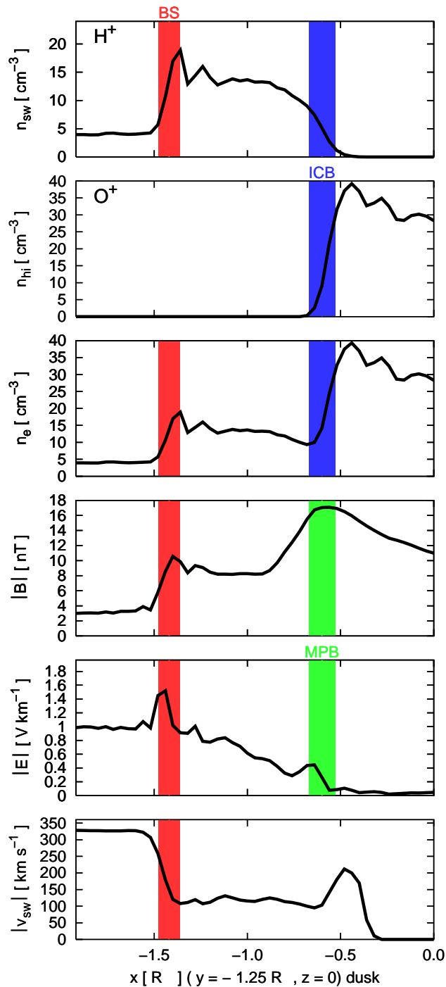
Fig. 11. Simulation results for the “standard run”. Plasma and field parameters along a line parallel to the x-axis in the equatorial plane at y = -1.25 R_M and z = 0 (straight white line in Fig. 10). These results should be compared to the measurements made by Phobos-2 in Fig. 2. The figure shows the number density of the solar wind protons and the planetary O^+ ions, the electron density, the magnetic and the electric field absolute values and the velocity of the solar wind, respectively. The color bars indicate the location of the BS (red), ICB (blue) and MPB (green). The magnetic field and electron density are in good agreement with the observed data. The proton density measured by Phobos-2, however, shows a pronounced foot region, which is not present in our results, due to a differing field geometry described in the text. The interplanetary electric field decreases after the bow shock and vanishes inside of the ICB. However, a small peak just in front of the ICB can be seen. The proton velocity remains constant behind the bow shock but it is increased directly behind the ICB. The very low proton density at this point indicates that only the fastest thermal solar wind protons are able to cross the boundary, leading to this increasing of the bulk velocity. The MPB and ICB are located at the same position, which is in accordance to the Phobos-2 observations.
