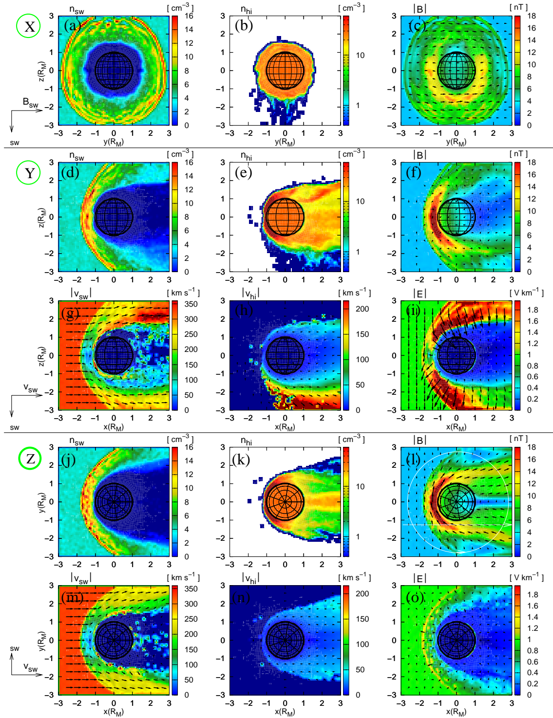
Fig. 10. Simulation results for the “standard run” for three orthogonal cross sections through the simulation box. (a), (d), (j) solar wind density, (b), (e), (k) heavy ion density, (c), (f), (l) magnetic field and vectors, (g), (m) solar wind bulk velocity, (h), (n) heavy ion bulk velocity and (i), (o) electric field, for the respective cutting planes from Fig. 3. The white lines in panel (l) correspond to the one-dimensional cuts of Figs. 11 and 12. The density plots show a clear separation of solar wind ions and heavy ions (ICB). The convective electric field \mathbf{E} = -\mathbf{v} \times \mathbf{B} vanishes, where the plasma of the heavy ions dominates. The magnetic field piles up at the planet’s dayside and reaches a maximum value (MPB), where the ICB is located. On the nightside the slow, heavy ions form several rays; below the south pole a fast component of pick-up ions is present. The bow shock exhibits some shocklet substructuring. See text for details. Parameters: same as in Fig. 7 at t=1169 s.
