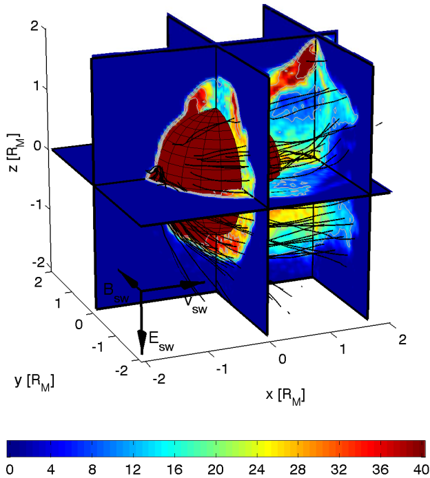
Fig. 8. Simulation results for the “standard run” continued. The cutting planes show the heavy ion density ( O^+ ) in \text{cm}^{-3} . The black solid lines represent the streamlines of the corresponding velocity field. The heavy ions form a complex tail structure behind the planet. Note the boundary on the dayside, where the heavy ion density shows a sharp increase. This is also the case for the upper edge of the ion tail in the E^- hemisphere (above the north pole), whereas in the E^+ hemisphere the boundary is not that pronounced. If one compares this to Fig. 7, the sharply bounded tail fits exactly into the solar wind plasma wake. Hence, both ion species are completely separated. This boundary is the “ion composition boundary” (ICB). Inside the tail the heavy ion density becomes asymmetric, as is seen at the plane x=5/3 R_M . The heavy ions form rays inside the tail. The flow pattern is much more asymmetric with respect to the equatorial plane compared to the solar wind flow pattern. Beneath the south pole some cycloidal motion of a large gyroradius can be seen, whereas in the rest of the tail region the stream lines are bundled inside the tail rays. Furthermore, a wave-like structure with rather large amplitude is evolved on the dayside at the ICB in the E^- hemisphere (north pole). This wave strips off heavy ion plasma clouds with high density. This structure is non-stationary. Parameters: see Fig. 7.
