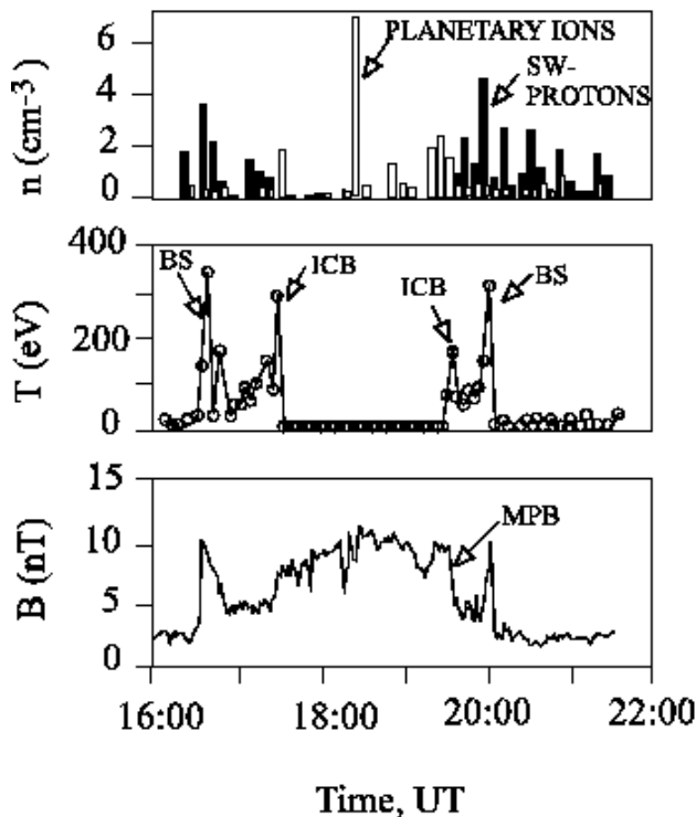
Fig. 1. Number density of the solar wind protons and heavy ions, proton temperature and magnetic field along a circular orbit from 16 March 1989 measured by ASPERA on board Phobos-2 (adapted from Sauer and Dubinin, 2000). In the plasma wake of the planet no solar wind protons are observed (proton cavity). The ion composition boundary (ICB) separates the solar wind protons from the planetary ions in this orbit. The sharp decrease of the proton temperature shows a clear feature of this boundary. At the same position a magnetic pile-up boundary (MPB) can be seen.
