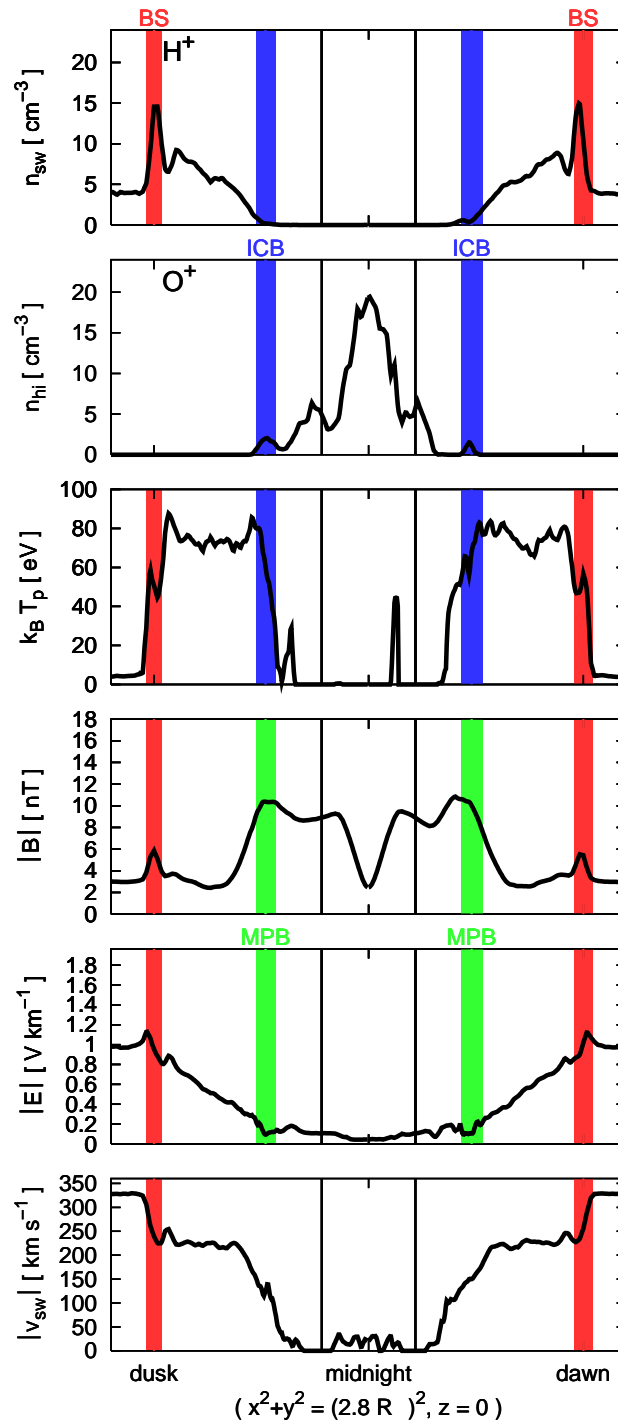
Fig. 12. Simulation results for the “standard run”. Plasma and field parameters along a circular orbit at 2.8 R_M around Mars in the plane z=0 . This should be compared to the data of the circular Phobos-2 orbit in Fig. 1. The black vertical lines mark the crossing of the optical shadow. The colored bars have the same meaning as in Fig. 11. The heavy ion tail is split up in the plasma sheet with high density and four tail rays with smaller densities (see also Fig. 16c). The near midnight rays are located at the minima of the overall magnetic field. This anti-correlation can also be seen from the observed data of Fig. 1. The proton temperature drops down at the ICB, which is also in agreement with Phobos-2 data.
