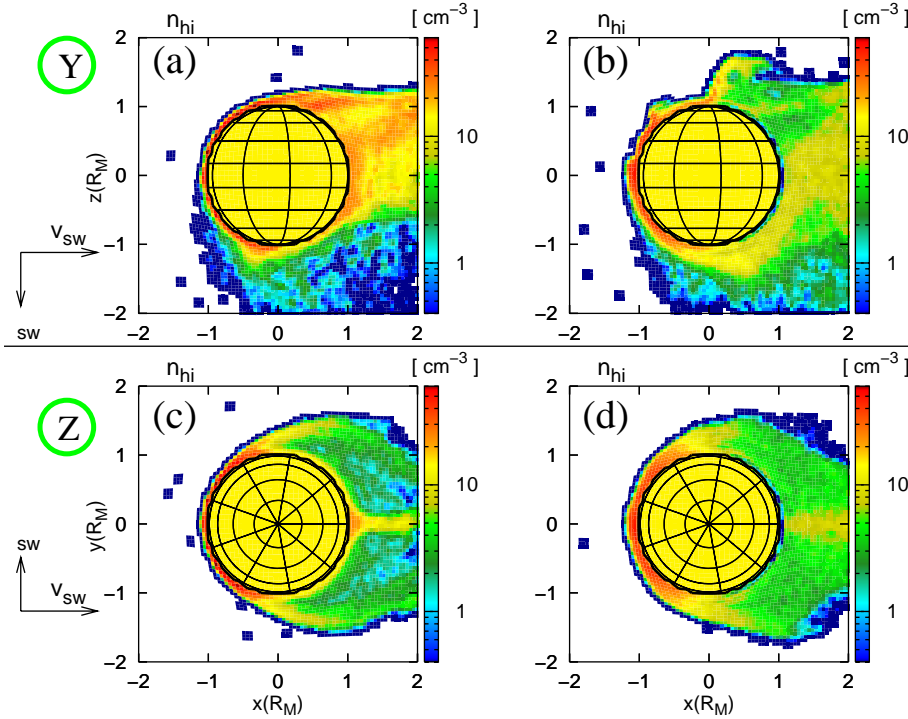
Fig. 15. Heavy ion distribution around Mars for two different electron temperatures inside the ionosphere. (a) and (c) T_{e,h}=2\cdot 10^4 K (nominal temp.). (b) and (d) T_{e,h}=1\cdot 10^5 K (increased temp.). The ion production rate Q is half of the standard run value. The increased temperature for the heavy ions shifts the ICB farther upstream. The tail rays become less sharp. The wave instability in the E^- hemisphere above the north pole becomes more pronounced. Parameters: t=1058 s, \nu=1\cdot 10^{-7} s ^{-1} , n_{sw}=4 cm ^{-3} .
