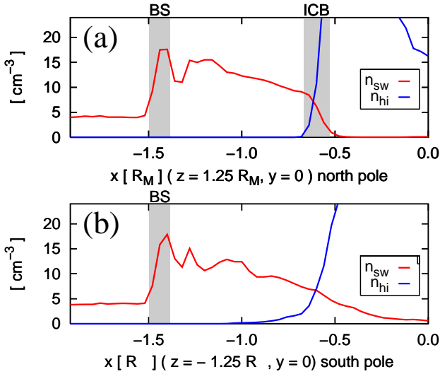
Fig. 13. Cuts along a line parallel to the x -axis in the polar plane at (a) z=1.25 R_M (850 km above north pole) and (b) z=-1.25 R_M (850 km below south pole). The ICB, which is clearly developed in the E^- hemisphere (a) cannot be seen in the E^+ hemisphere (b). This results from the different orientation of the electric field in both hemispheres, pointing inwards towards the ionosphere, above the north pole and outwards below the south pole, see also Fig. 10i. Parameters: see Fig. 7.
