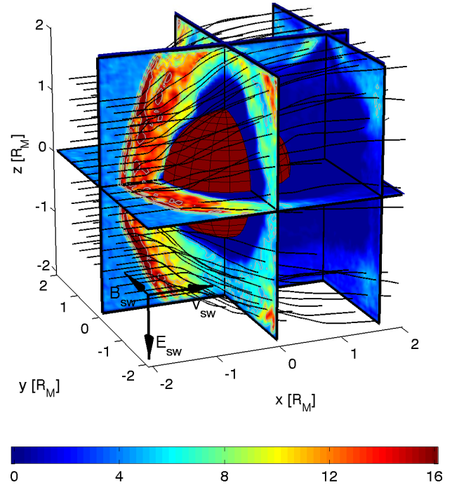
Fig. 7. Simulation results for the “standard run”. The cutting planes show the solar wind density in \text{cm}^{-3} . The black solid lines represent streamlines of the corresponding velocity field. The solar wind flows almost symmetrically around the obstacle. On the nightside, a plasma wake is formed, where the solar wind density vanishes almost completely. This wake region, however, is not symmetric with respect to the equatorial plane, as can be seen from the cutting plane at x = 5/3 R_M . Downstream of the bow shock, a multiple shocklets structure is obvious.
