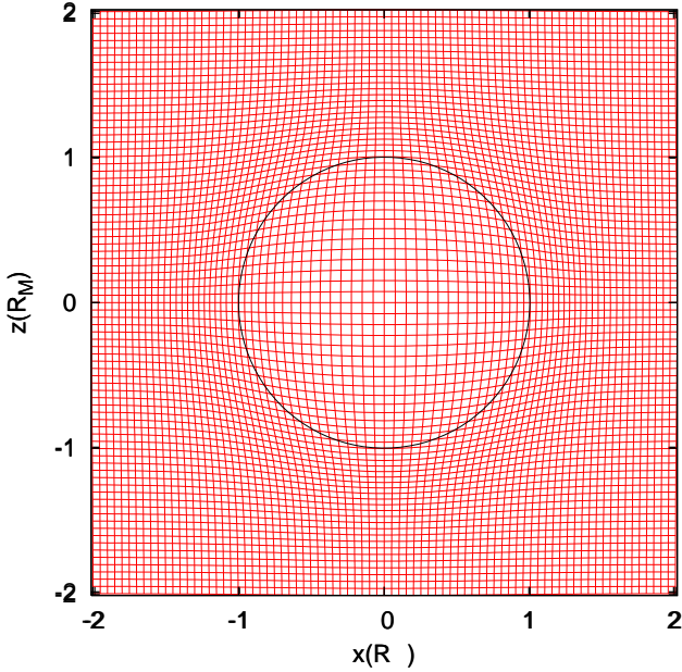
Fig. 4. Structure of the simulation grid used. A cross section through the box is shown with \alpha=0.21 , \beta=0.37 and \gamma=7.07 (see text) consisting of 80 \times 80 cells in the plane y=0 . This grid used for the actual simulation runs, gives a higher resolution near the Martian surface (black circle) compared to the outer cells.
