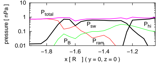
Fig. 14. The distribution of the kinetic pressure of the solar wind ( P_{\text{ram}} ), thermal pressure of the solar wind ( P_{\text{sw}}=P_{e,sw}+P_i ), thermal pressure of the heavy ion plasma ( P_{\text{hi}}=P_{e,hi}+P_{hi} ), and magnetic pressure ( P_B ) along the Sun-Mars line on the dayside for the “standard run”. Parameters: see Fig. 7.
