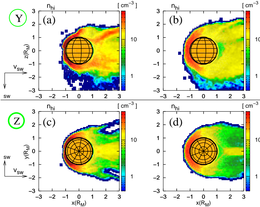
Fig. 16. Heavy ion distribution around Mars for two different solar wind densities. (a) and (c) n_{sw}=4 cm ^{-3} (standard run parameter). (b) and (d) n_{sw}=2 cm ^{-3} . The ICB shifts outward with decreasing solar wind density. Decreasing the density of the solar wind is equivalent to increasing the production rate of the heavy ions. This figure, together with Fig. 15, shows that the thermal electron pressure n_e k_B T_{e,h} inside the ionosphere is the crucial parameter for the location of the ICB. Parameters: t=835 s, \nu=2\cdot 10^{-7} s ^{-1} , T_{e,h}=2\cdot 10^4 K.
