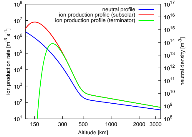
Fig. 5. Neutral gas density (blue line), the ion production rate (red line in subsolar direction and green line at the terminator) of oxygen as a function of altitude at solar minimum ( v=1 \cdot 10^{-7} \text{ s}^{-1} ). Note the two different axis scales.
