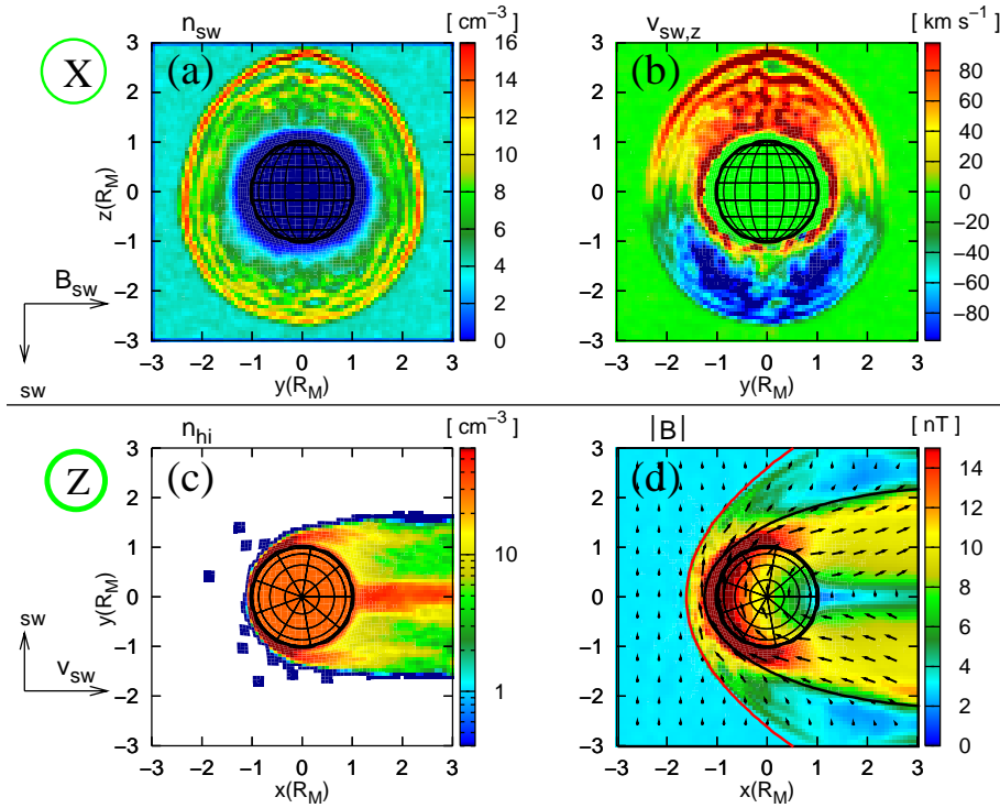
Fig. 17. Comparison of the simulated boundaries with Mars Global Surveyor data. (a) solar wind density, (b) z -component of the solar wind velocity in the plane x=0 , (c) heavy ion density and (d) magnetic field in the plane z=0 . The red (BS) and black (MPB) solid lines in panel (d) represent a fit with Eq. (10) obtained from the MGS data, which is taken from Vignes et al. (2000). This good agreement between simulation and observation was achieved for a value of T_{e,h}=3000 K, which is about the measured temperature of the dominant O^+ component in the Martian ionosphere (Hanson and Mantas, 1988). Parameters: t=1545 s, v=2\cdot 10^{-7} s ^{-1} , T_{e,h}=3\cdot 10^3 K (low temp.), n_{sw}=4 cm ^{-3} .
