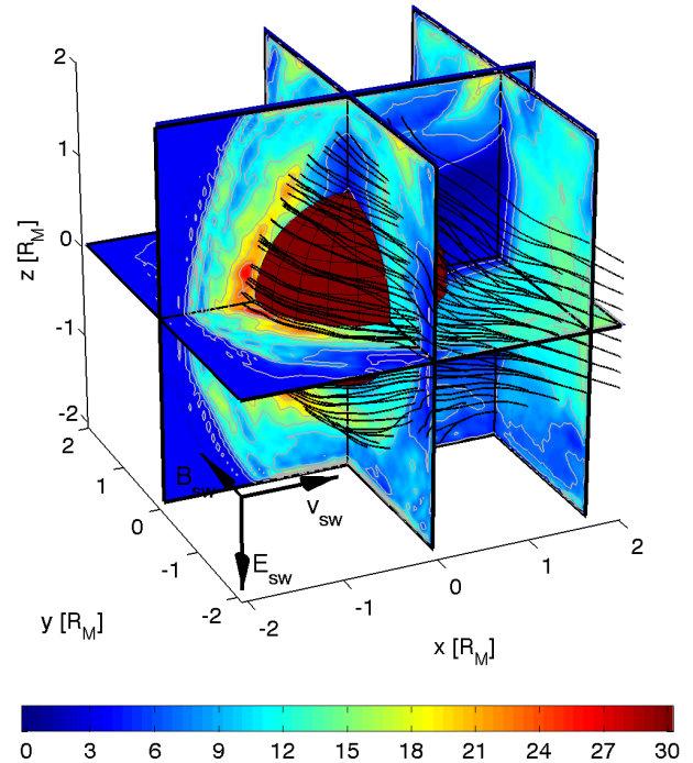
Fig. 9. Simulation results for the “standard run” continued. The cutting planes show the magnetic field in nT. The black solid lines represent the magnetic field lines. The magnetic field lines are draped around the obstacle. Just in front of the ICB, the magnetic field reaches its maximum, which indicates the “magnetic pile-up boundary” (MPB). The magnetic field vanishes inside the wake in the polar plane. The full three-dimensional structure in the tail is again highly asymmetric and complicated. The same shocklet substructuring as in Fig. 7 can be seen downstream of the BS. Parameters: see Fig. 7.
