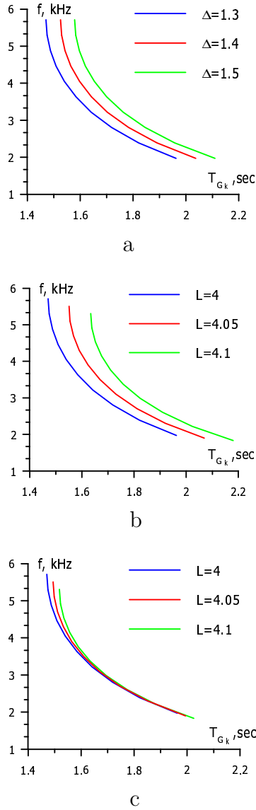
Fig. 6. The group delay time of the first eigenmode propagating from the eautor to the ionosphere in the different ducts:
