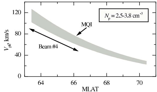
Fig. 9. Estimates of the meridional Pc3–4 wave phase velocity for the model in Fig. 8 (dipole magnetic field, magnetopause proton density N_p = 2.5\text{--}3.8 cm ^{-3} , N_p(r) \propto 1/r^4 ).
