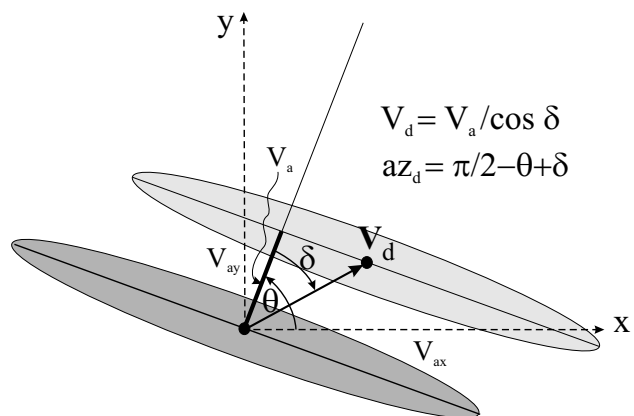
Fig. 10. Motion of elongated absorption patch. The initial (final) patch position is shown by the dark (light) ellipse. The velocity of apparent motion (perpendicular to the longest patch dimension) V_a is obtained from the apparent velocities along the axes V_{ax} and V_{ay} .
