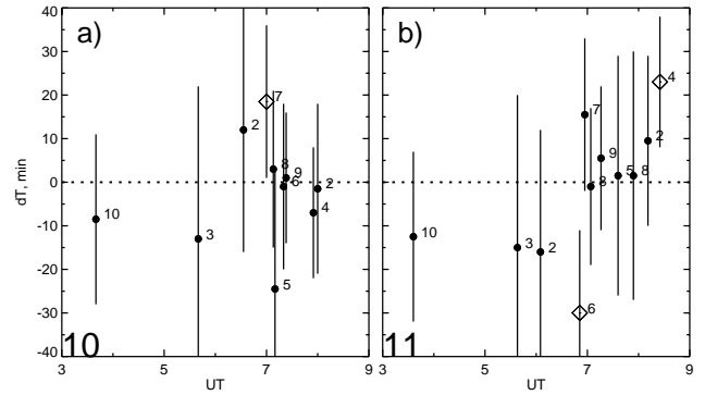
Fig. 5. The time difference between the motion direction reversals as determined from two different methods versus the reversal time from the second method: (a) from the absorption images and keograms and (b) from the absorption images and magnetic perturbations. The total number of points is indicated in the bottom left corner of each panel. The diamonds mark the points that are farther from the zero time difference than the estimate uncertainty (vertical bars). The digits by each point indicate the event number from Table 1.
