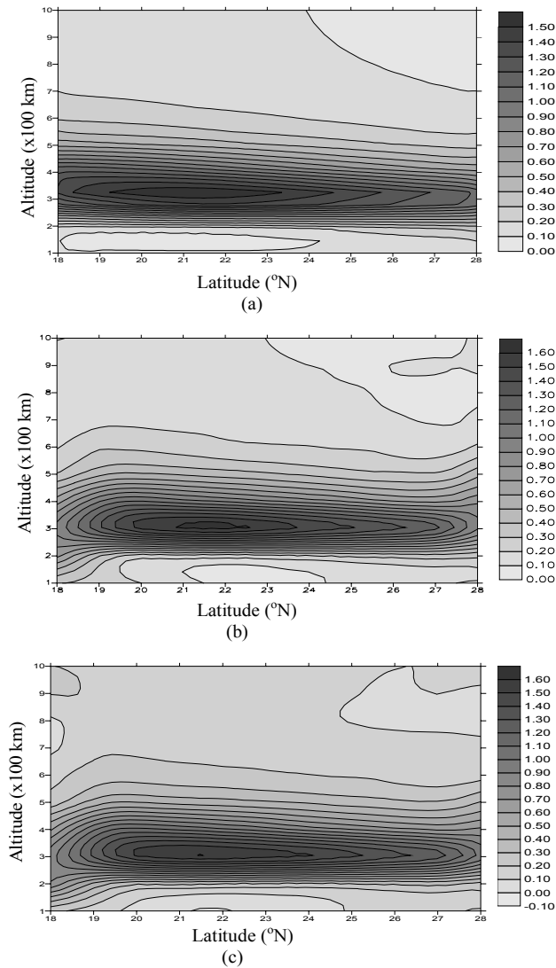
Fig. 1. (a) Electron Density ( 10^6 \text{ cm}^{-3} ) distribution obtained from IRI 2001 (b) GSVSD reconstruction using 220 ray paths (c) reconstruction with 250 ray paths.
