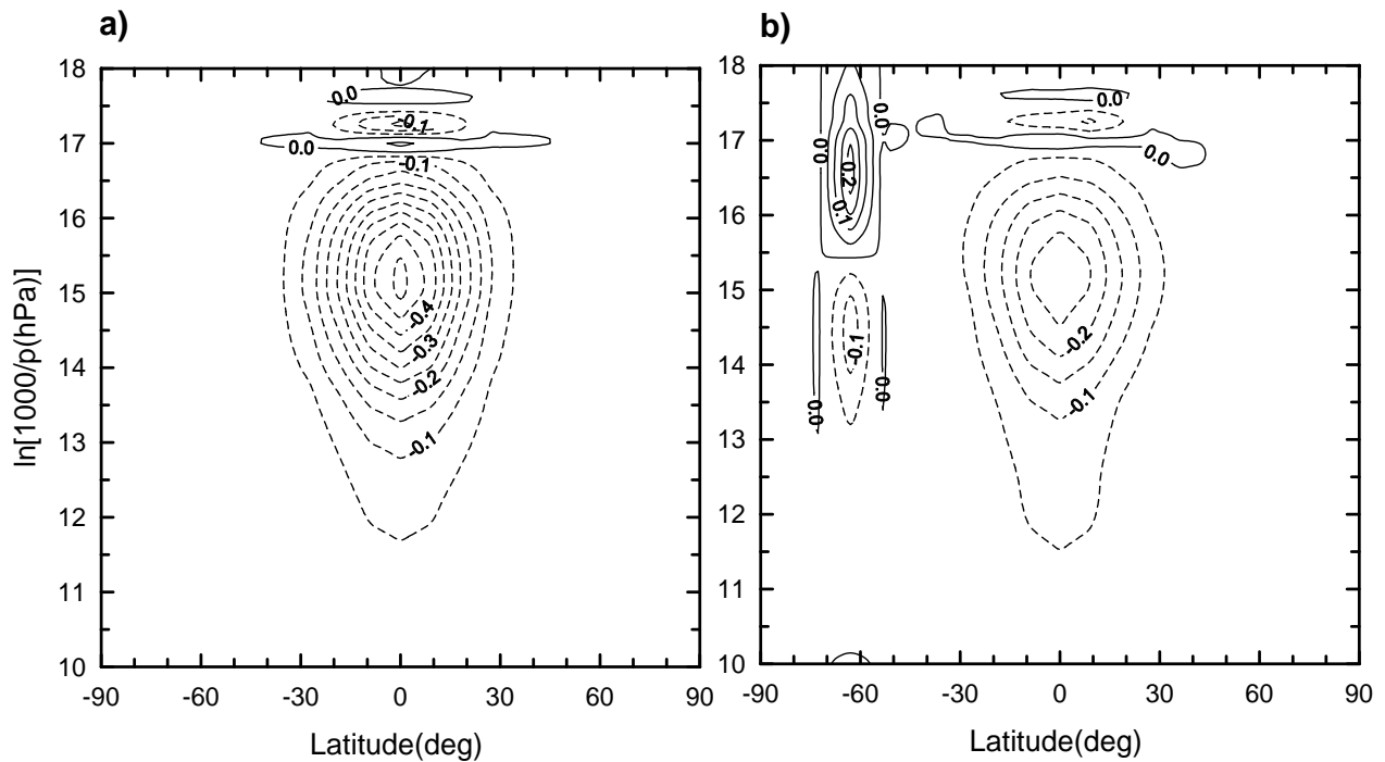
Fig. 10. Latitude-height distributions of change in heat influx in K/day due to perturbations of the \text{CO}_2 15- \mu\text{m} emission during propagation of the ultra-fast Kelvin wave for 16 March (a) and 1 July (b). The dashed isolines correspond to increasing the cooling rate.
